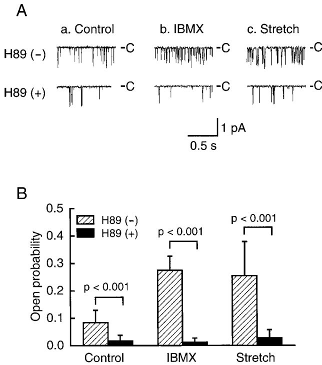
FIGURE 7. Effects of H89 on the P_o of the basal, IBMX-, and stretch-activated NSC channels obtained in cell-attached patches formed on the apical membrane at no applied potential (the resting membrane potential). (A) Representative traces of the single channel currents obtained from the basal (a, Control), IBMX-activated (b, IBMX), and stretch-activated (c, Stretch) channels with and without H89 pretreatment (0.5 \mu M, 2 h). H89 decreased the P_o of the channel in each case. (B) The statistical result of the effects of H89 on the P_o of the basal (Control), IBMX-activated (IBMX), and stretch-activated (Stretch) channels. In all the basal, IBMX-, and stretch-activated NSC channels, the P_o of the NSC channel was significantly decreased by the treatment of H89. n = 11 .
