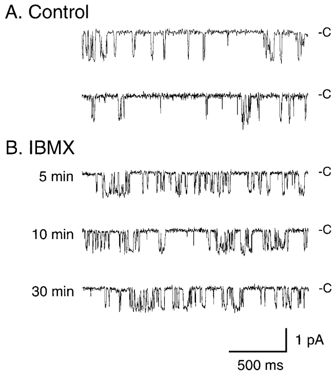
FIGURE 1. Single-channel currents. These currents were obtained from a cell-attached patch formed on the apical membrane with no applied potential (i.e., the resting apical membrane potential) in IBMX-untreated (A, Control) and -treated (B) cells. Closed level of single channel within patch is marked with a horizontal bar and “C” to the right of the trace. Downward deflection indicates inward current across the patch membrane. IBMX (1 mM) increased the P_o of the channel. IBMX (1 mM final concentration) was added to the basolateral solution.
