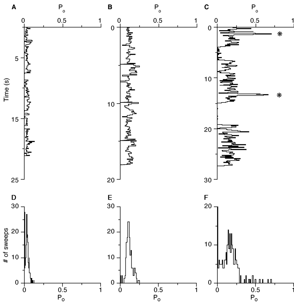
FIGURE 12. Effect of Bay K8644 on the open probability of the channel. Channel P_o of 100 ms segments from recordings at continuous depolarization plotted against time (A–C). (D–F) Histograms of P_o values for the periods shown in A–C. The first and probably second bin of each distribution represent segments with no detectable openings (28 and 6 in D, 3 and 0 in E, 63 and 4 in F). Recordings from a patch under control conditions at +60 mV (A and D) and +70 mV (B and E) and in the presence of 50 \mu M Bay K8644 (C and F) at +60 mV constant depolarization. The asterisks in C mark clusters with 4 and 5 consecutive high P_o sweeps (see text).
