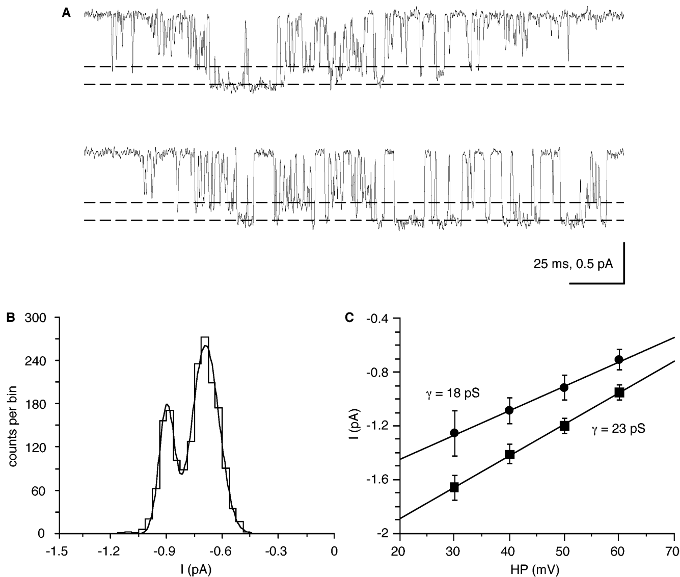
FIGURE 10. Multiple conductance levels in the presence of Bay K8644 (50 \mu M). (A) Two sample records (0.25 s) during steady +60 mV depolarization which show large amplitude long-duration openings and short-duration openings of smaller amplitude. The dashed lines indicate the two conductance levels of the open channel. Records were filtered at 1.5 kHz. (B) Distribution of single-channel current amplitudes at +60 mV depolarization, fitted by the sum of two Gaussians. (C) Plot of single-channel conductances which were determined from linear least-squares fits of the mean single-channel current amplitudes. The error bars denote the standard deviation of the Gaussian fits. All potentials are relative to the cell's resting membrane potential.
