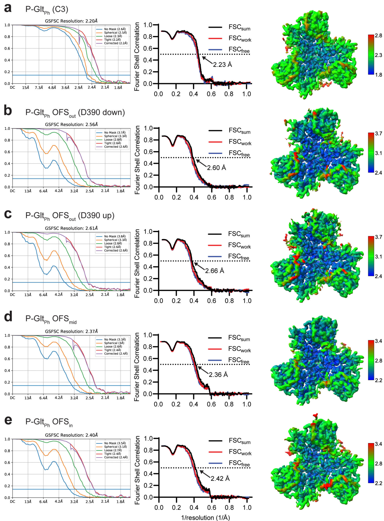
Figure S10. Validation statistics for models from Data S2. (a–e) OFS-C3 (a); OFS out D390 down (b); OFS out D390 up (c); OFS mid (d); OFS in (e). From left to right, map FSC from NU-refinement in cryoSPARC, model-to-data validation in Phenix of the trimer, and local resolution estimation. All maps are contoured at 8 \sigma except a, which is contoured at 10 \sigma . The top protomer in b–e is the subject of focused classification and model refinement.
