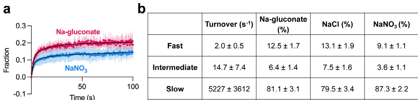
Figure S4. Fitted parameters of L-Asp uptake by WT Glt ph in the presence of various anions. (a) Aspartate transport of Glt ph (C321A/N378C) was measured using the single-transporter FRET-based assay in NaNO 3 (blue) or Na-gluconate (red). Data are means and SE from three independent experiments performed as in Fig. 2 f. (b) Data in a and Fig. 2 f were fitted to triexponential functions (a three-phase association model; GraphPad Prism). Initial and final fractions of total possible uptake were set to 0 and 1, respectively. The three turnover rates (fast, intermediate, and slow), corresponding to the heterogeneous transporter populations, were constrained to be the same for all datasets (see Materials and methods for a detailed description of data processing). Three independent experiments per condition were analyzed, and values shown are means and SEM of the fitted parameters.
