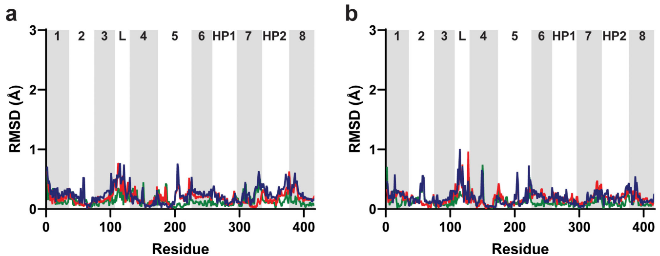
Figure S12. Protomers adjacent to chain A do not display concerted movements. Trimers were aligned along the trimerization regions of all three protomers (residues 150–195). (a and b) Per-residue C \alpha RMSDs of chain B (a) and chain C (b). Lines are OFS out /OFS mid (green); OFS mid /OFS in (red); and OFS out /OFS in (blue). Transmembrane domains are labeled and alternatively shaded. L, the disordered loop between domains 3 and 4.
