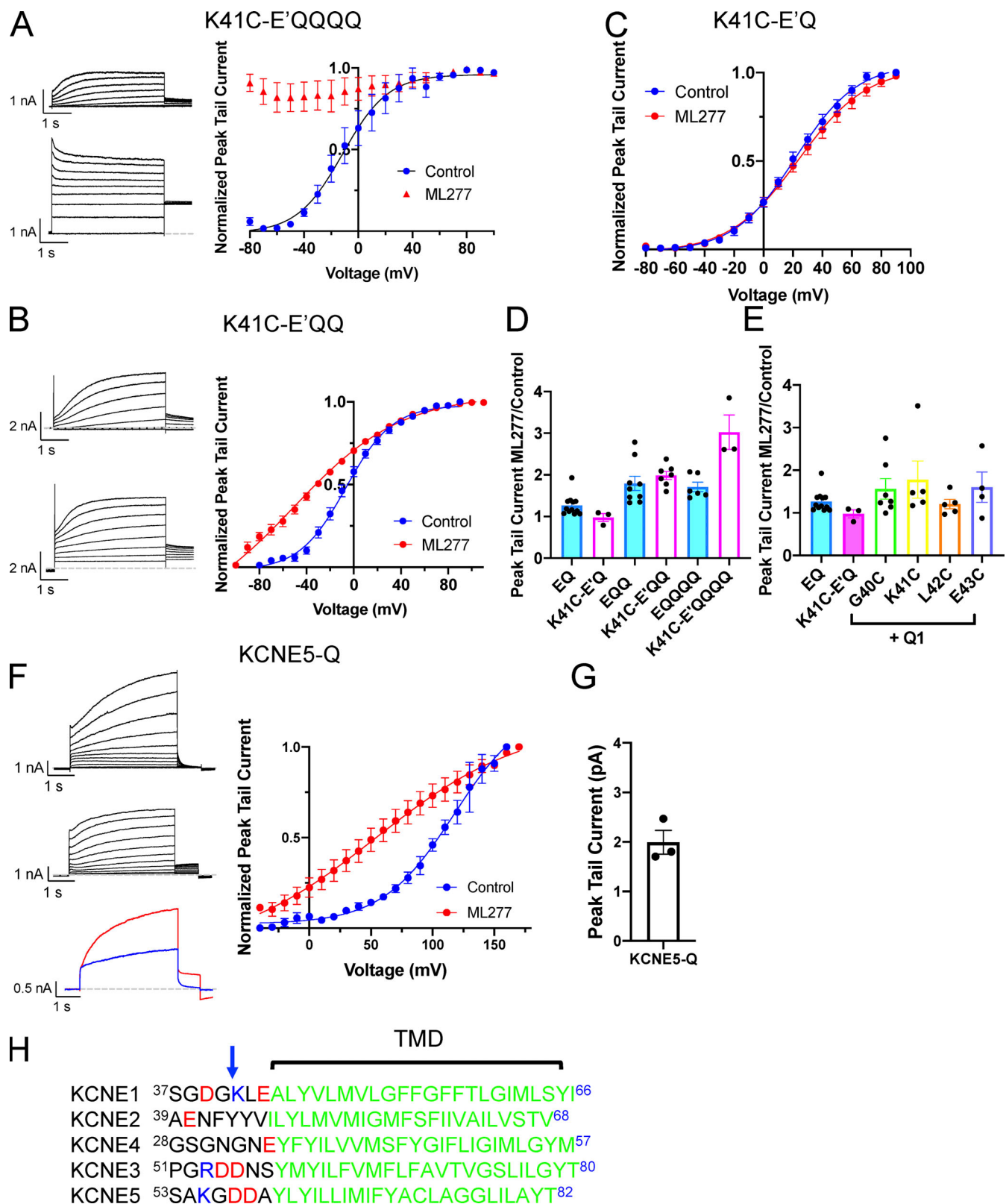
Figure 8. The K41C mutation in KCNE1 allows ML277 to activate I_{Ks} as long as the complexes are not fully saturated. (A) Representative whole-cell currents of K41C-E'QQQ obtained using a voltage-clamp protocol before (top) and after 1 \mu M ML277 (bottom). Cells were held at -90 and pulsed from -90 to +100 in 10-mV steps for 4 s, then to -40 mV for 0.9 s. The interpulse interval was 15 s. Only even voltages are shown for clarity. The graph on the right shows the G-V plots ( n = 3 ). (B) Representative whole-cell currents of K41C-E'QQ obtained using the same activation protocol as described in A. The upper record is before ML277, and the lower trace is after 1 \mu M ML277 was added to the bath. The graph on the right shows the G-V plots ( n = 4 or 5). (C) G-V plots for K41C-E'Q in control conditions and in 1 \mu M ML277 ( n = 4 or 5). (D) Bar chart shows the tail current amplitude in ML277 divided by control amplitude for WT channel
