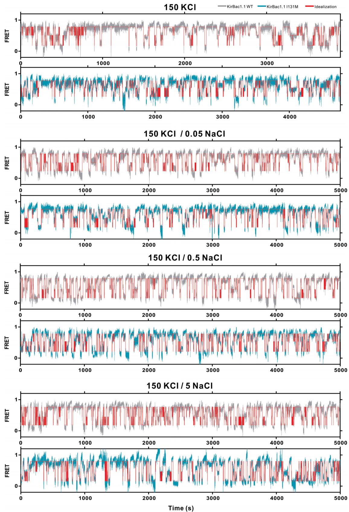
Figure S4. Low \text{Na}^+ -dependent kinetics of SF in KirBac1.1 WT and I131M. Concatenated smFRET trajectories of WT (gray) and I131M (green) in 150 mM KCl with zero \text{Na}^+ , 0.05 mM \text{Na}^+ , 0.5 mM \text{Na}^+ , or 5 mM \text{Na}^+ , as indicated, together with three state idealizations (red) corresponding to low, middle, and high FRET states.
