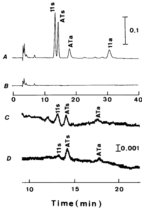
FIGURE 3. Analysis of isomers of 3-hydroxyretinal by HPLC for the homogenates of heads of carotenoid-rich (A) and carotenoid-deficient (B, C, and D) flies. 20 mg head homogenate was analyzed in A and B. Elution peaks of the syn isomers 11- cis (11s) and all- trans (ATs) 3-hydroxyretinaloxime, and the anti isomers all- trans (ATa) and 11- cis (11a) 3-hydroxyretinaloxime, are indicated. (C) and (D) HPLC analysis using 140 mg of homogenates of heads of carotenoid-deficient flies monitored at a higher sensitivity of the ultraviolet detector. The homogenates were irradiated with an intense 460-nm light, and then with 581-nm light (C) or just with 460-nm light alone (D) before the formation of oximes. Same scales for A and B, C and D.
