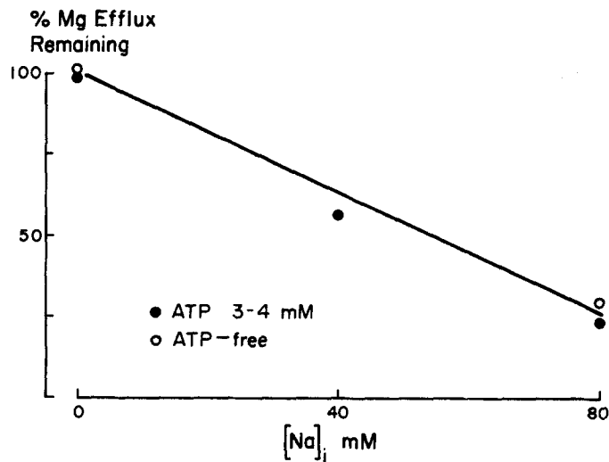
FIGURE 6. This shows the effect of changes in [Na]_i on Mg efflux in the presence or absence of ATP_i .
