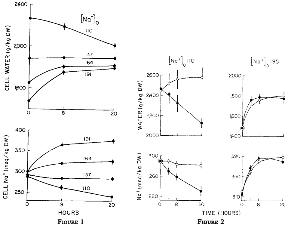
FIGURE 1. Cell water and sodium content as a function of incubation time at 37°C. Media contained sodium in the concentrations (millimolar) shown with each line, plus (mM): bicarbonate 25, glucose 10, calcium 5, chloride = anion remainder. All media contained bovine serum albumin 1 g/100 ml, and all suspensions were gassed with 95% O 2 -5% CO 2 . pH was 7.3-7.4 at 37°C. Mean ± SEM for four studies.
