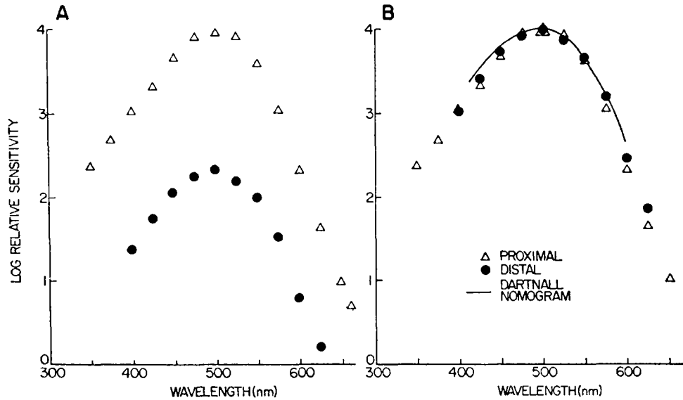
FIGURE 6. Spectral sensitivities of proximal and distal cells. In B the curve from the distal cell shown in A was shifted upward by 1.7 log unit. A Dartnall nomogram curve for a pigment with a \lambda_{max} = 500 nm is shown in B.
