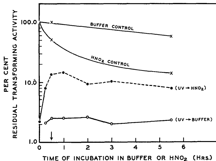
FIGURE 5. Nitrous acid reactivation of ultraviolet-irradiated denatured C_{25} DNA. Effect of time of incubation. UV irradiation, see the section on Methods. Concentration of denatured DNA 40 \mu\text{g/ml} , time, 100 seconds. \text{HNO}_2 or buffer treatment, 1 M nitrite in 0.05 M acetate buffer or buffer alone, initial pH 4.8, concentration of denatured DNA, 20 \mu\text{g/ml} , time is indicated in the figure, temperature, 37^\circ\text{C} . The upper signs (x) show the control values of samples without irradiation treated with acetate buffer or \text{HNO}_2 during 0.5 or 5.5 hours. The arrow over the time axis indicates the time of treatment of samples in most of the other experiments.
