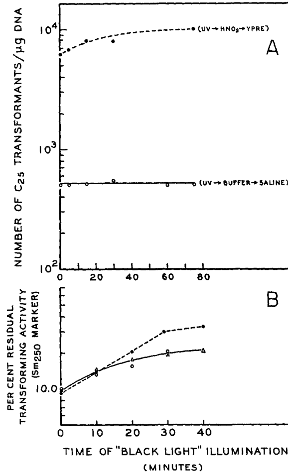
FIGURE 8A. Photoreactivation after nitrous acid reactivation conditions of this experiment. See the legend of Fig. 7B.
