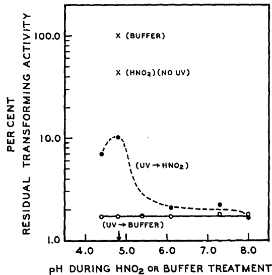
FIGURE 3. Effect of pH on nitrous acid reactivation of ultraviolet-irradiated denatured C_{25} DNA. UV irradiation, see the section on Methods. Concentration of denatured DNA, 40 \mu\text{g}/\text{ml} ; time, 100 seconds. \text{HNO}_2 or buffer treatment, pH 4.4 to 6.1, 1 M nitrite in 0.05 M acetate buffer or the buffer alone; pH 7.3 and 8.0, 1 M nitrite in 0.01 M phosphate buffer or the buffer alone; initial pH is indicated in the figure, concentration of denatured DNA 20 \mu\text{g}/\text{ml} ; time, 30 minutes, temperature, 37°C. After this the samples with pH between 4.4 and 6.1 were neutralized by a tenfold dilution with 0.02 M \text{Na}_2\text{HPO}_4 in 0.3 M NaCl. The samples at pH 7.3 or 8.0 were diluted tenfold with 0.01 M citrate in 0.3 M NaCl. The final pH oscillated between 7.2 to 7.6. The upper signs (x) show the control values of samples without UV irradiation treated with acetate buffer or \text{HNO}_2 , pH 4.8. The arrow over the pH axis indicates the pH during most of the other experiments.
