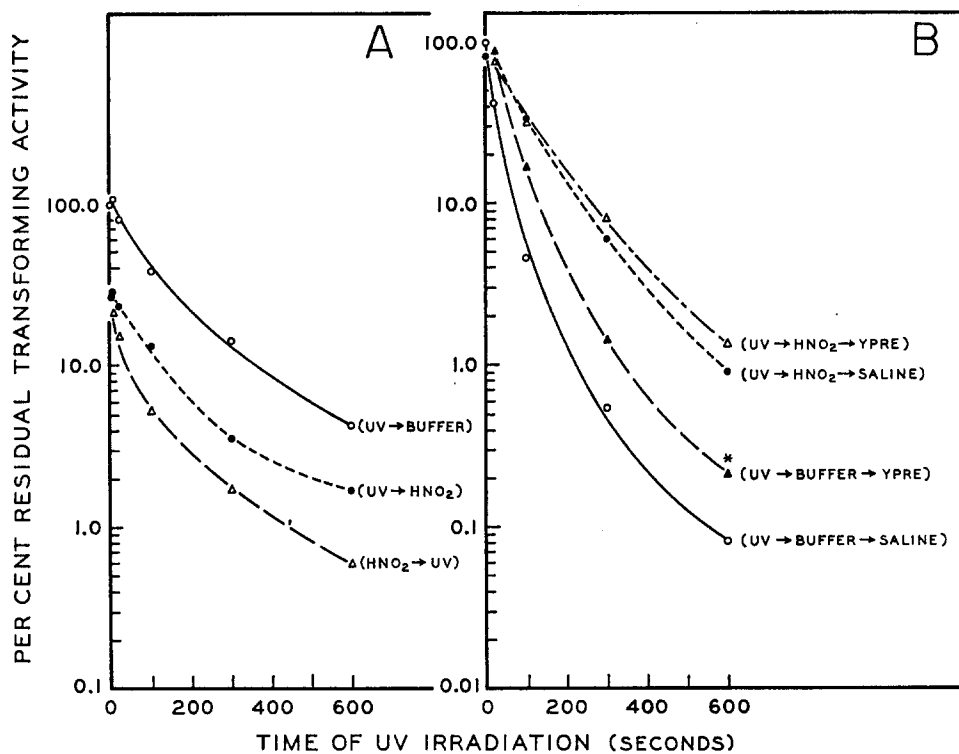
FIGURE 7A. Nitrous acid on ultraviolet-irradiated denatured E 20 DNA. UV irradiation, see the section on Methods. Concentration of denatured E 20 DNA, 100 \mu g/ml. HNO 2 or buffer treatment, 1 M nitrite in 0.05 M acetate buffer or buffer alone, initial pH 4.8, concentration denatured E 20 DNA, 50 \mu g/ml, time, 30 minutes, temperature, 37°C.
