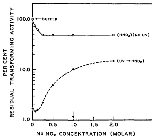
FIGURE 4. Nitrous acid reactivation of ultraviolet-irradiated denatured C_{25} DNA. Effect of the concentration of nitrite. UV irradiation, see the section on Methods. Concentration of denatured DNA, 40 \mu\text{g/ml} , exposure, 100 seconds. \text{HNO}_2 or buffer treatment, different concentration of nitrite in 0.05 \text{ M} acetate buffer or the buffer alone; initial pH in the presence of 1 \text{ M} nitrite was 4.8. Concentration of denatured DNA 20 \mu\text{g/ml} , time, 30 minutes, temperature, 37^\circ\text{C} . The upper arrow shows the control value of a sample without irradiation treated with acetate buffer. The arrow over the concentration axis indicates the nitrite concentration at which most of the other experiments were made.
