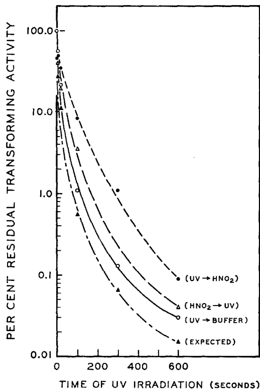
FIGURE 1. Nitrous acid reactivation of ultraviolet-irradiated denatured C 25 DNA. UV irradiation, see the section on Methods. Concentration of denatured DNA, 100 \mu g/ml. HNO 2 or buffer treatment, 1 M nitrite in 0.05 M acetate buffer or the buffer alone; initial pH 4.8; concentration of denatured DNA 50 \mu g/ml; time, 30 minutes, temperature, 37°C. Expected curve, it was calculated as 50 per cent of the control (UV buffer) curve at each point (see text).
