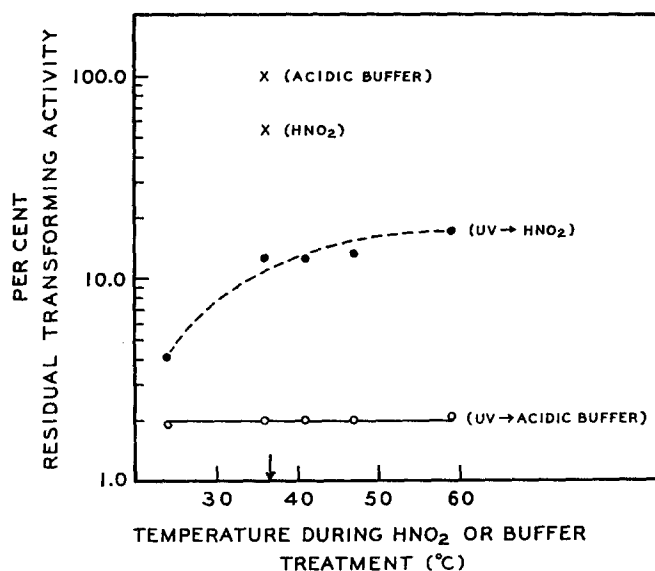
FIGURE 2. Effect of temperature on the nitrous acid reactivation of ultraviolet-irradiated denatured C_{25} DNA. UV irradiation, see the section on Methods. Concentration of denatured DNA, 40 \mu\text{g}/\text{ml} ; time, 100 seconds. \text{HNO}_2 or buffer treatment, 1 M nitrite in 0.05 M acetate buffer or the buffer alone, initial pH 4.8; concentration of denatured DNA 20 \mu\text{g}/\text{ml} ; time, 30 minutes, temperature as indicated in the figure. The upper signs (x) show the control values of samples without UV irradiation treated with buffer or \text{HNO}_2 at 36°C. The arrow over the temperature axis indicates the temperature at which most of the other experiments were made.
