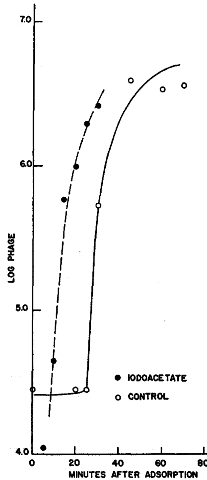
FIG. 5. Addition of m/1000 iodoacetate at intervals during latent period of phage 14 in M. aureus 145.
