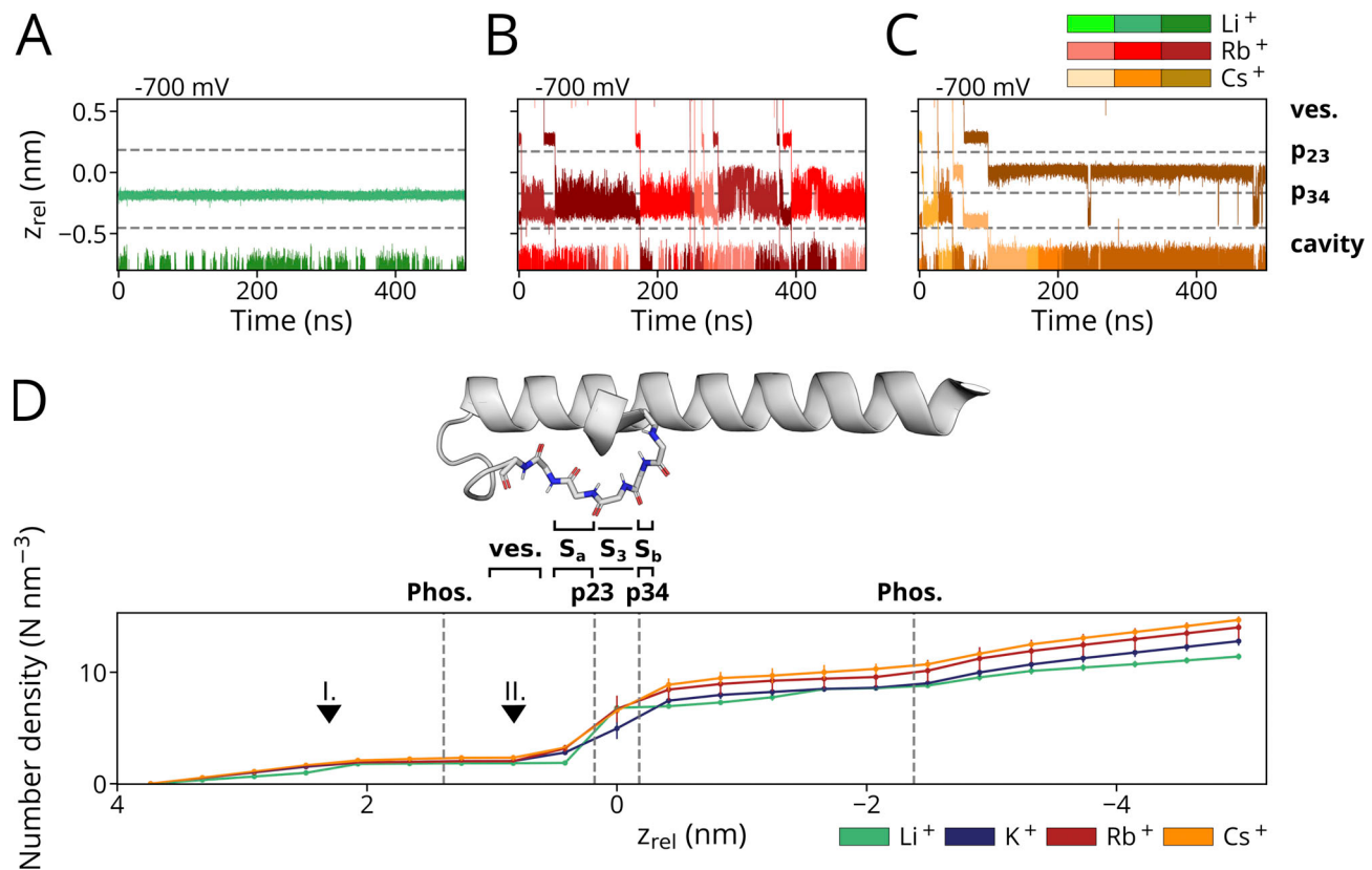
Figure 2. Characteristic ion trajectories depicting primary binding sites of \text{Li}^+ , \text{Rb}^+ , and \text{Cs}^+ obtained from simulations conducted at -700 mV in solutions with a single cation species. (A) With prolonged presence of \text{Li}^+ , p34 was identified as a single binding site within the SF. Permeation of \text{Li}^+ through p23 was only observed in a single instance. (B) Similar to \text{K}^+ , \text{Sa} (encompassing p23) and \text{Sb}/\text{Sc} (proximate to p34) were identified as binding sites within the SF for \text{Rb}^+ . Intermediate fluctuations between \text{Sb} and \text{S3} in the single-ion state are observable at higher voltages, while prolonged binding to \text{S3} occurred at lower voltages. (C) \text{Cs}^+ is predominantly found as a single cation in the \text{S3} site in all simulations. Both \text{Rb}^+ as well as \text{Cs}^+ are found in a \{\text{Sa}, \text{Sc}\} configuration during conduction events. (D) Empirical CDF of computed numerical densities (in counts/nm 3 ) for \text{Li}^+ , \text{Rb}^+ , and \text{Cs}^+ conducted at -700 mV ( n = 4 , n = 1 , and n = 2 , respectively), including simulations depicted in A–C and of \text{K}^+ ( n = 4 ; pure KCl), and \text{Rb}^+ ( n = 3 ; pure RbCl) at -500 mV along the z -axis of the simulation box. The mean z positions of p23, p34, and the POPC-headgroup phosphor atoms (Phos.) are marked as dashed lines. Arrowheads denote reference z_{\text{rel}} positions along the pore axis: Unequal count densities are observed for \text{Li}^+ compared to the other cations (I.), whereas similar number densities are observed in the vestibule above the SF (II.). For reference, the channel pore-facing helix and the SF of a single HCN4 monomer are shown above the subplot. The vestibule (ves.) and SF binding sites \text{Sa} , \text{S3} , and \text{Sb} are separately outlined.
