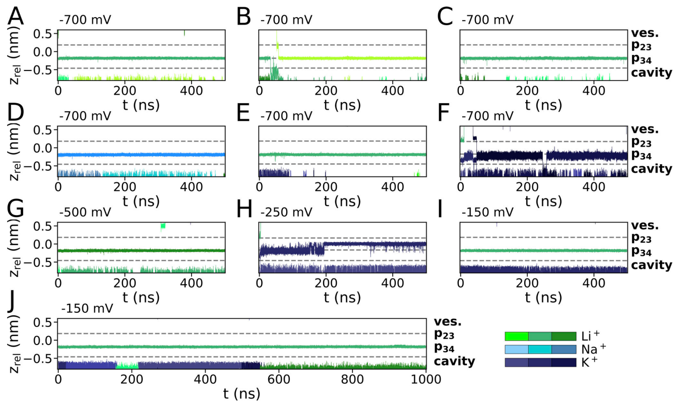
Figure S1. Ion trajectories for simulations with \text{Li}^+/\text{Na}^+ and \text{K}^+ (900 mM) at various membrane voltages. (A–F) Hyperpolarizing voltages of -700 mV were applied for pure LiCl with \text{Li}^+ preplaced in p34. (D–F) Simulations were conducted at the same voltage and mixed-cationic sets for (D) LiCl/NaCl with \text{Na}^+ preplaced in p34, (E) LiCl/KCl with \text{Li}^+ preplaced in S3, (F) LiCl/KCl with \text{Li}^+ and \text{K}^+ preplaced in p23 and p34, respectively. (G–J) Additional simulations at lower hyperpolarized membrane potentials with initial placement (G) of \text{Li}^+ in p34 and within the cavity, (H) \text{Li}^+ in p23 and \text{K}^+ in p34 and (I and J) \text{Li}^+ in p34 were conducted with -500 , -250 , and -150 mV, respectively.
