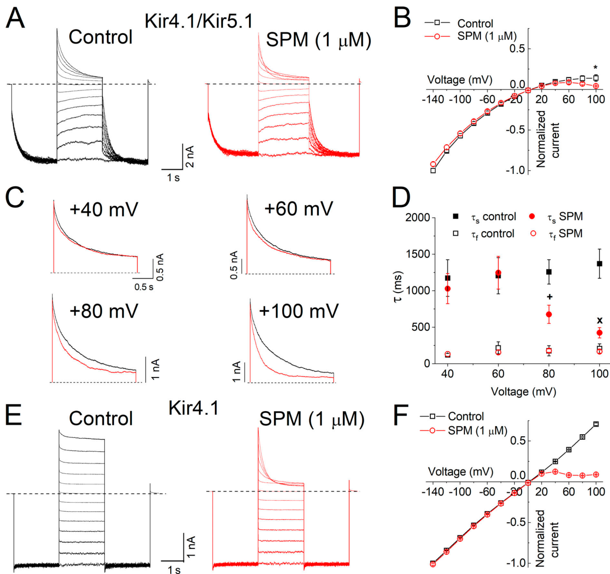
Figure 3. Effect of exogenous SPM on inside-out Kir4.1/Kir5.1 and Kir4.1 currents. (A) Kir4.1/Kir5.1 currents before (control) and after perfusing 1 μM SPM in the bath. Currents were recorded in the inside-out configuration applying the same triple-pulse voltage protocol as for Fig. 2. (B) Normalized I-V relationships for Kir4.1/Kir5.1 in the absence (control) and presence of 1 μM SPM. Currents were measured at the end of the test pulses and normalized to the amplitude of the current recorded at -140 mV in control conditions. (C) Superimposed Kir4.1/Kir5.1 current traces from A illustrating control currents (black traces) and their respective SPM-induced block (red traces) at +40, +60, +80, and +100 mV. (D) Time constants ( \tau_{\text{slow}} [ \tau_s ] and \tau_{\text{fast}} [ \tau_f ]) of Kir4.1/Kir5.1 currents as shown in C, in control conditions and in the presence of 1 μM SPM. (E and F) Current recordings (E) and normalized I-V relationships (F) for Kir4.1 in control and after 1 μM SPM, obtained as described for A and B, respectively. The dashed line denotes the zero-current level. Data are presented as mean \pm SEM. n = 5 for Kir4.1/Kir5.1 and n = 11 for Kir4.1. *, P = 0.047 ; +, P = 0.032 ; x, P = 0.029 .
