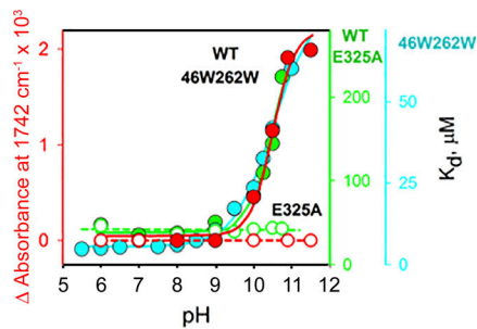
Figure 4. pK a of Glu325 in LacY. The pH dependence of \Delta -IR intensity change at 1742 cm -1 was measured with the LacY G46W/G262W mutant in the absence or presence of \alpha -NPG (filled red circles) or E325A LacY (open red circles). The K_d values for \alpha -NPG binding to WT LacY (filled green circles), E325A LacY (open green circles), or LacY G46W/G262W mutant (filled cyan circles) were calculated as the ratio of rate constants ( k_{off}/k_{on} ) measured by stopped-flow fluorescence.
