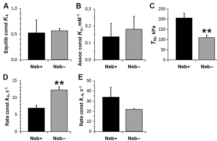
Figure 8. The kinetic constants of steps 4 and 5, and T_{56} , deduced from the effect of Pi on 2pb and tension. (A) K_4 is the equilibrium constant of the force generation step 4. (B) K_5 is Pi association constant (step 5). (C) T_{56} is fiber tension when all CBs are either at AM*DP or AM*D states, and scales with force/CB. (D) k_4 is the forward rate constant of the force generation step 4. (E) k_{-4} is its backward rate constant. n = 7 for Neb + fibers, and n = 8 for Neb - fibers. Assoc, Association; Equilib, Equilibrium; const, constant.
