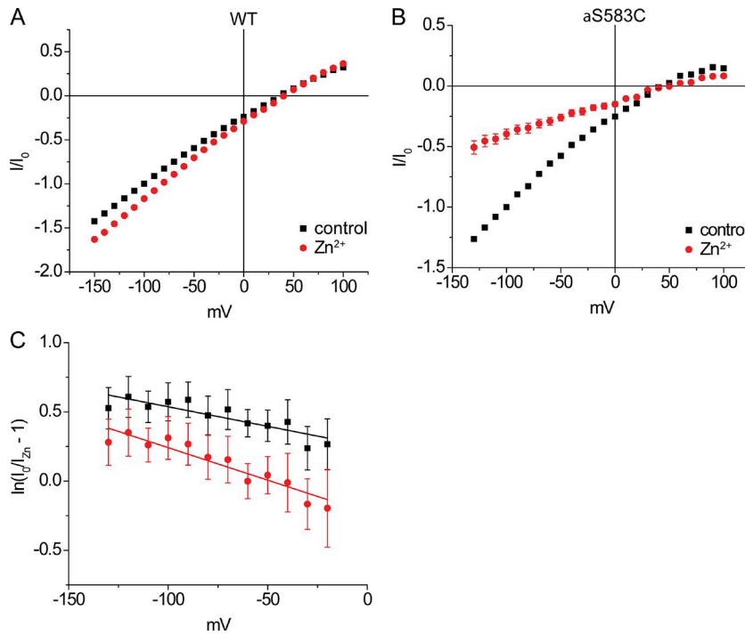
Figure 11. Voltage dependence of block by \text{Zn}^{2+} in oocytes expressing \alpha\text{S583C}/\beta/\gamma ENaC. (A) I_{\text{Na}}-V relationships for WT ENaC in 110 mM NaCl with no \text{Zn}^{2+} and 0.2 mM \text{Zn}^{2+} . (B) I_{\text{Na}}-V relationships for ENaC \alpha\text{S583C}/\beta/\gamma in 110 mM NaCl with no \text{Zn}^{2+} and 0.2 mM \text{Zn}^{2+} . (C) Plot of \ln(I_0/I_{\text{Zn}} - 1) versus voltage, where I_0 and I_{\text{Zn}} are currents in the absence and presence of \text{Zn}^{2+} , respectively, for \alpha\text{S583C}/\beta/\gamma . The slope of the relationship obtained by linear regression gives K_{\text{Zn}}(0) = 230 \pm 40 \mu\text{M} , z \cdot \delta = 0.14 \pm 0.01 ( n = 5 ), assuming no stimulation of the channel by \text{Zn}^{2+} (red). Analysis assuming the same activation of WT and \alpha\text{S583C}/\beta/\gamma gives K_{\text{Zn}}(0) = 150 \pm 20 \mu\text{M} , z \cdot \delta = 0.06 \pm 0.01 (black).
