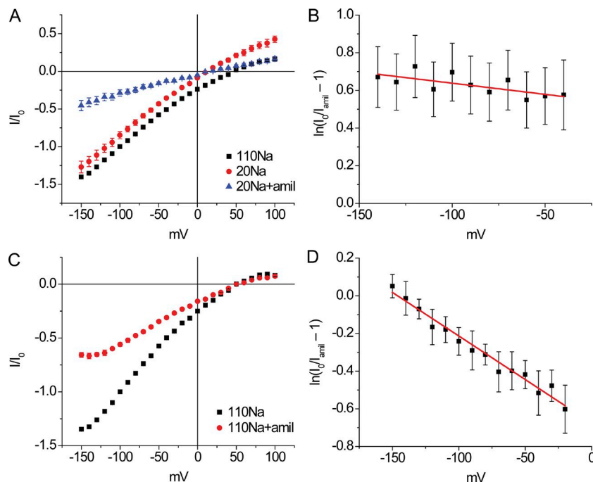
Figure 12. Voltage dependence of block by amiloride in oocytes expressing WT and \alpha\text{S583C} ENaC. (A) I_{\text{Na}}-V relationships for WT in 20 mM NaCl with no amiloride or 0.1 \mu\text{M} amiloride (amil). (B) Plot of \ln(I_0/I_{\text{amil}} - 1) versus voltage where I_0 and I_{\text{amil}} are currents in the absence and presence of amiloride, respectively. The slope of the relationship obtained by linear regression gives K_{\text{amil}} = 64 \pm 11 \text{ nM} , z \cdot \delta = 0.03 \pm 0.01 ( n = 6 ). (C) I_{\text{Na}}-V relationships for \alpha\text{S583C} in 110 mM NaCl with no amiloride or 10^{-6} \text{ M} amiloride. (D) Plot of \ln(I_0/I_{\text{amil}} - 1) versus voltage. The slope of the relationship obtained by linear regression gives K_{\text{amil}} = 2.0 \pm 0.2 \mu\text{M} , z \cdot \delta = 0.12 \pm 0.01 ( n = 4 ).
