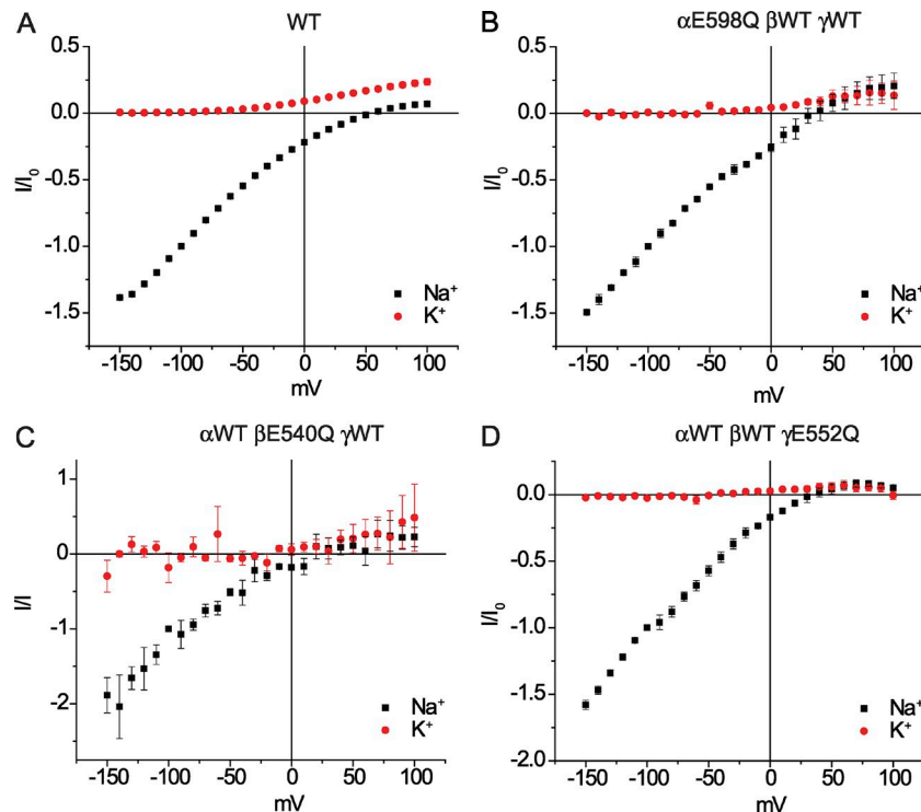
Figure 4. Current-voltage relationships in the presence of 110 mM Na + and 110 mM K + in oocytes expressing ENaC with mutations in the E21' positions. (A) WT. (B) αE598Q/βWT/γWT. (C) αWT/βE540Q/γWT. (D) αWT/βWT/γE552Q. All data are corrected for amiloride-insensitive currents and normalized to the value at V_m = -100 mV in the presence of Na + ( I_0 ). Data represent means \pm SEM for three to seven oocytes.
