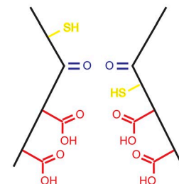
Figure 1. Alignment of the C-terminal transmembrane domains of human ASIC1a and rat ENaC subunits. The putative GAS selectivity region, named for the amino-acid sequence in ASIC1, is marked in blue, the conserved acidic amino acids in red, and the sites of \text{Zn}^{2+} -sensitive cysteine locations in yellow. Bottom: The transmembrane segments in one subunit of the putative open structure of chicken ASIC (Baconguis et al., 2014; PDB accession no. 4NTW), and a cartoon representation of the transmembrane pore. The relevant elements in TM2 are indicated with the same color scheme.
