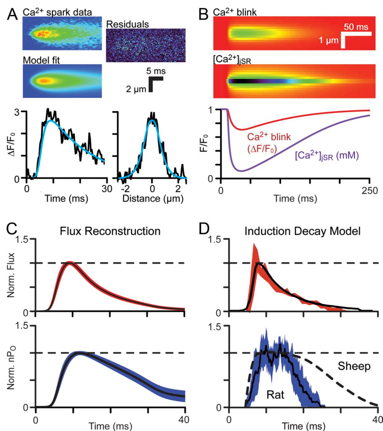
Figure 3. Estimating jSR \text{Ca}^{2+} depletion and RyR gating time course by flux reconstructions. (A) The 3-D model of \text{Ca}^{2+} reactions, diffusion, and microscope blurring shown in Fig. 2 generates a \text{Ca}^{2+} spark record, which is fitted to experimental data by varying a basis function for the jSR permeability time course (Kong et al., 2013). (B) Although not fitted, the model can also calculate the corresponding SR \text{Ca}^{2+} depletion signals, which are similar to those recorded experimentally (Brochet et al., 2005). (C) From the calculated release flux (red) and the jSR \text{Ca}^{2+} levels, the jSR permeability time course was derived (normalized flux in red and normalized n\text{Po} [number of open channels] in blue). (D) Normalized release flux (red) and permeability (blue) changes from the induction decay model of Cannell et al. (2013). Note the concordance of flux estimates by both models, although the permeability time course is dependent on species-dependent RyR \text{Ca}^{2+} sensitivity.
