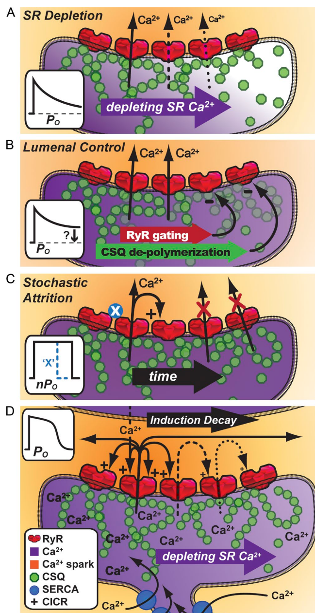
Figure 1. Possible CICR termination mechanisms. (A) SR \text{Ca}^{2+} depletion. A reduction in SR \text{Ca}^{2+} levels will reduce release flux regardless of RyR gating (as described by their open probability, P_0 ). However, fateful termination by this mechanism alone is problematic, because the jSR lumen is continually refilled from the rest of the SR. (B) SR luminal control of RyR gating may be modulated either by a direct effect on the RyR itself (red) and/or via an accessory protein such as CSQ (green). However, the extent to which these mechanisms could reduce RyR P_0 sufficiently to terminate release is unclear. (C) Stochastic attrition. If all RyRs close simultaneously, then the release flux is terminated. However, it is unlikely that this will occur within the timescale of a \text{Ca}^{2+} spark. Stochastic attrition could be accelerated by coupled gating between RyRs, either by direct contact or by a protein linker (X). (D) Induction decay. After CRU activation, jSR \text{Ca}^{2+} levels decline which results in a decreasing release flux. The local cytoplasmic \text{Ca}^{2+} level is proportional to the release flux, and this is transduced via the steep \text{Ca}^{2+} dependence of
