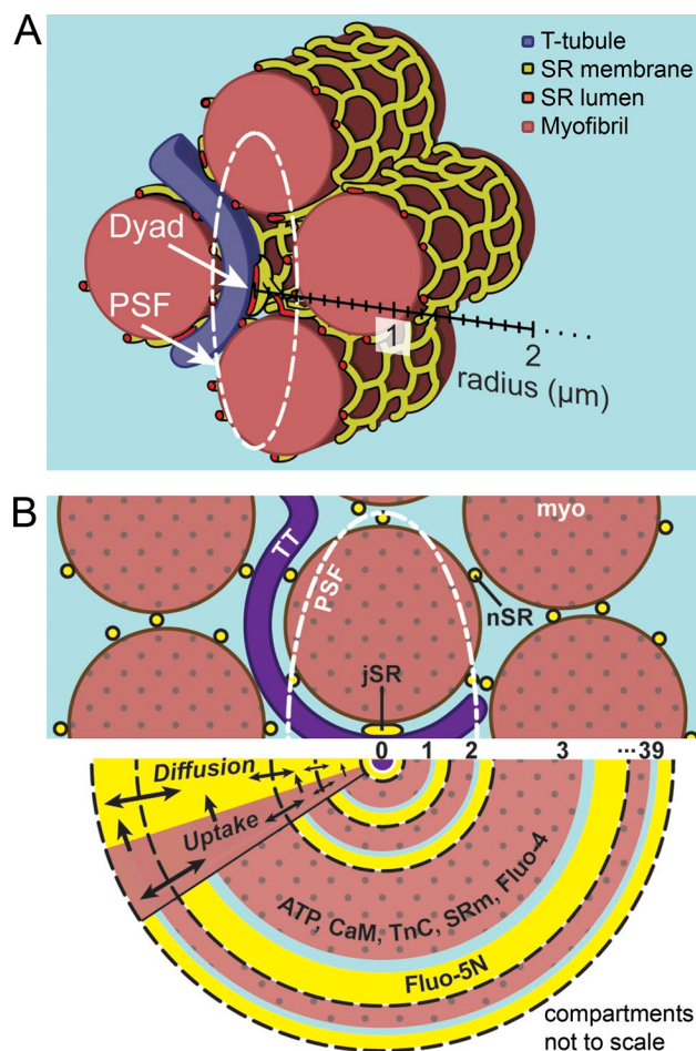
Figure 2. A method for calculating jSR release fluxes from spark records. (A) A simplified diagram illustrating the relative sizes of the T-tubules, jSR, network SR (nSR), myofibrils (myo), and a typical microscope PSF that blurs the \text{Ca}^{2+} signals. (B) By using spherical geometry for the model, the computational complexity is greatly reduced while still retaining the volume fractions and concentrations of each component that contribute to \text{Ca}^{2+} fluxes. Effectively, the spatial geometries of each component are spread over each computational compartment, making transport from the jSR isotropic at the length scale of interest (200 nm). The center element is dedicated to the dyadic space (including the jSR with CSQ; Kong et al., 2013), and all other compartments include reaction and diffusion fluxes in the cytosol and SR as indicated in the bottom part of the figure. Having calculated the spatial Fluo-4 and Fluo-5N signals, these are blurred by convolution with the microscope PSF, and the resulting signal is fitted to typical \text{Ca}^{2+} sparks by altering the time course of the jSR permeability change basis function (Kong et al., 2013). Because large numbers of simulations are performed to allow the release waveform to converge, efficiency in solving the discretized transport equations after microscope blurring is important.
