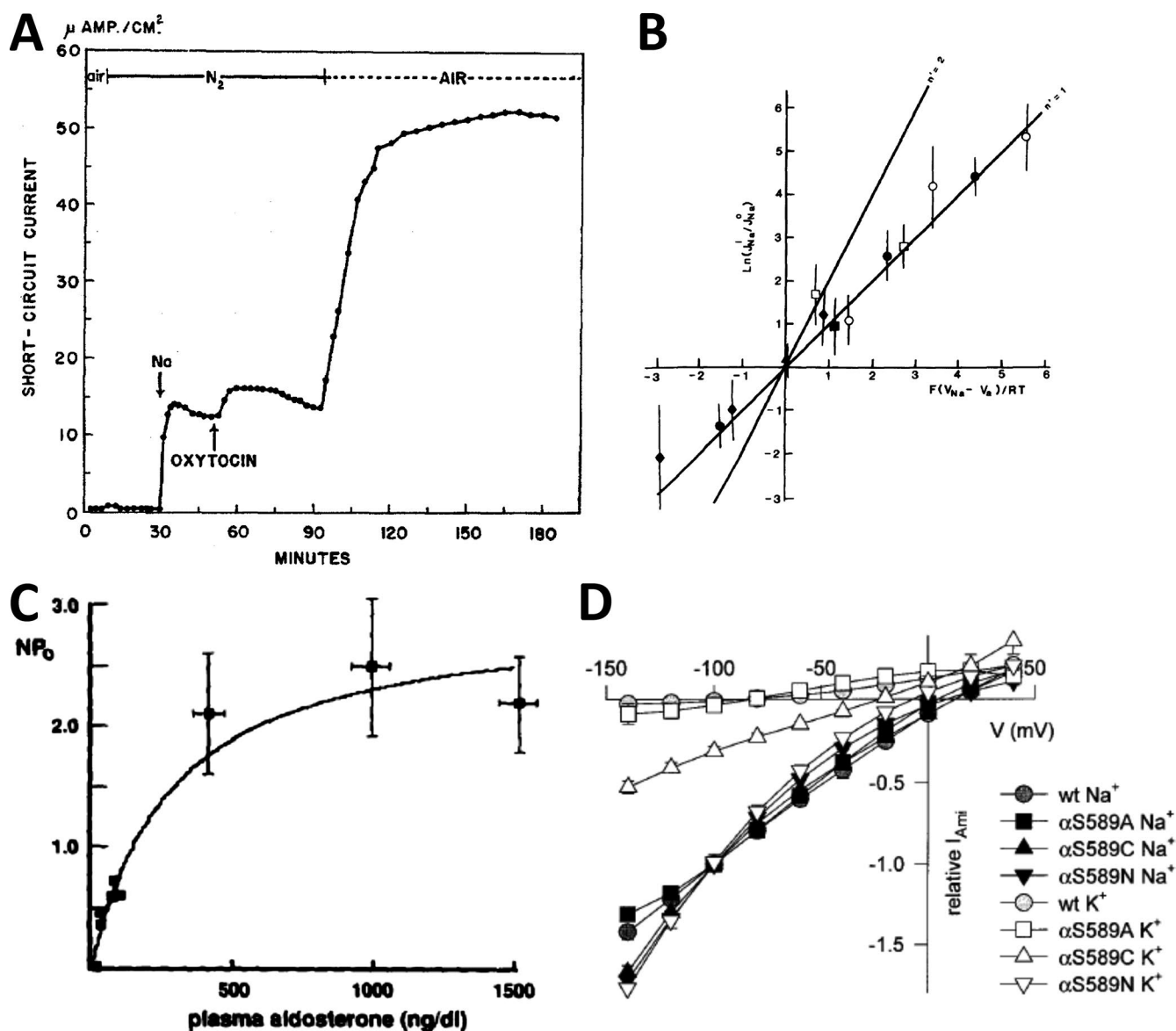
Figure 2. Epithelial \text{Na}^+ channels in absorptive epithelia. (A) Short-circuit current across the toad urinary bladder and its dependence on \text{Na}^+ and oxidative metabolism are shown. The short-circuit current under normal conditions was equal to the net flux of \text{Na} measured with \text{Na}^{22} and \text{Na}^{24} . Transport was stimulated by oxytocin or vasopressin and was enhanced in the presence of \text{O}_2 . From Leaf et al. (1958). (B) Flux-ratio analysis of \text{Na}^+ permeation in frog skin. The value n' = 1 is consistent with single-ion permeation through channels. From Benos et al. (1983). (C) Dependence of \text{Na}^+ channel activity on aldosterone in rat collecting duct. From Pácha et al. (1993). (D) Conduction through WT ENaC and channels with point mutations in the putative selectivity filter. The WT channel is almost perfectly selective for \text{Na}^+ , rather than \text{K}^+ , whereas mutations in the second transmembrane domain of the \alpha subunit confer conduction of \text{K}^+ . From Kellenberger et al. (2001).
