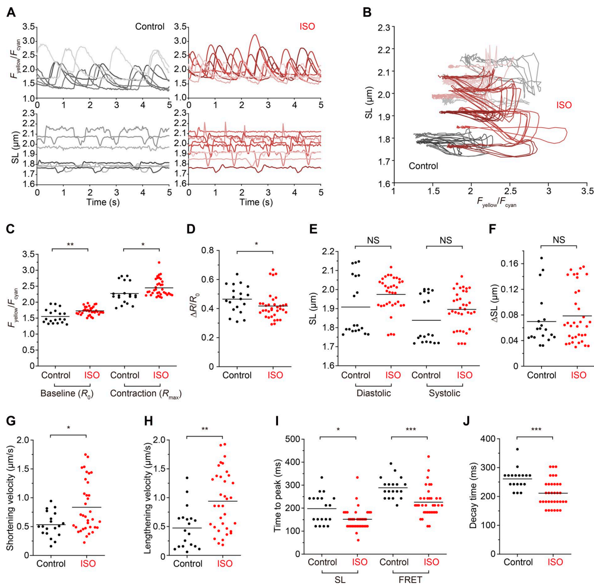
Figure 6. Effects of ISO on local coupling of [Ca^{2+}]_i and SL dynamics. (A) Individual data showing time courses of changes in F_{yellow}/F_{cyan} (top) and SL (bottom) in \alpha -actinin- YC -Nano140-expressing cardiomyocytes during spontaneous beating in the absence (left; indicated as "control") and presence (right) of 50 nM ISO. n = 7 and 9 in the absence and presence of ISO, respectively. Experiments were performed at 37^\circ C . (B) Individual data showing the relationship of F_{yellow}/F_{cyan} versus SL in the absence and presence of ISO. A closed loop-like trajectory was observed, regardless of the use of ISO (compare Butler et al., 2015). (C) Comparison of F_{yellow}/F_{cyan} values during relaxation ( R_0 ) and contraction ( R_{max} ) in the absence and presence of ISO. F_{yellow}/F_{cyan} was significantly higher for both R_0 and R_{max} . (D) Comparison of \Delta R/R_0 in the absence and presence of ISO (see Fig. 2 for \Delta R/R_0 ). (E) SL values in the absence and presence of ISO, during relaxation and contraction. ISO did not significantly affect SL, regardless of the contractile state. (F) \Delta SL (difference between SL at relaxation and contraction) values in the absence and presence of ISO. No significant difference was observed between groups. Likewise, the variance was similar for both groups (i.e., from \sim 0.03 to \sim 0.17 \mu m for control [difference, \sim 0.14 \mu m ] and from \sim 0.03 to \sim 0.15 \mu m for ISO [difference, \sim 0.12 \mu m ]). (G) Shortening velocity of SL dynamics in the absence and presence of ISO. The velocity became significantly faster in the presence of ISO. (H) Lengthening velocity of SL dynamics in the absence and presence of ISO. (I) Time to peak values for changes in F_{yellow}/F_{cyan} and SL in the absence and presence of ISO. The values were less for both parameters, indicating the acceleration of the EC coupling at the single sarcomere level. (J) Comparison of the decay time for F_{yellow}/F_{cyan} . The time was shorter in the presence of ISO, indicating enhanced removal of cytosolic [Ca^{2+}]_i , presumably via acceleration of SR Ca^{2+} pump coupled with PLN phosphorylation (see Bers [2001] and references therein). In all graphs, horizontal bars indicate mean values. *, P < 0.05 ; **, P < 0.01 ; and ***, P < 0.001 (Mann-Whitney U test).
