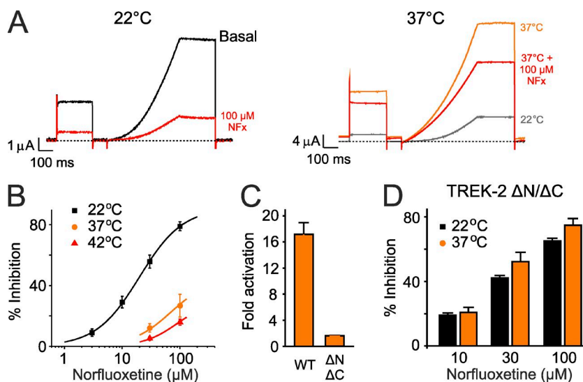
Figure 4. Temperature activation involves conformational changes in the TM helices. (A) Example traces showing temperature-dependent activation of whole-cell TREK-2 currents from 22^\circ C (left) to 37^\circ C (right) markedly decreases inhibition by 100 \mu M NFx. For comparison, the currents at 22^\circ C are also shown in gray in the right panel. Currents were recorded by voltage protocols similar to those used in Fig. 1 D. (B) Summary dose-response curves showing reduced NFx sensitivity of whole-cell TREK-2 currents at 22^\circ C , 37^\circ C , and 42^\circ C (data shown are percent inhibition of basal currents recorded at 0 mV; mean \pm SEM, n \geq 6 ). IC_{50} at 22^\circ C , 23.4 \pm 3.1 \mu M ; but at 37^\circ C and 42^\circ C , >100 \mu M . (C) A truncated version of TREK-2 (TREK2 \Delta N/\Delta C ) that no longer responds to temperature. Fold activation represents change in current between 22^\circ C and 37^\circ C . (D) The NFx sensitivity of this temperature-insensitive mutant is unaffected by temperature, indicating a specific effect on WT TREK-2. (C and D) Error bars shown are mean \pm SEM ( n \geq 6 ).
