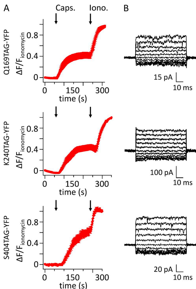
Figure 4. L-ANAP-incorporating TRPV1-TAG-YFP channels retain functional properties. Cells were cotransfected with pANAP and a plasmid encoding TRPV1-Q169TAG-YFP, TRPV1-K240TAG-YFP, or TRPV1-S404TAG-YFP, as indicated, and were cultured with L-ANAP-ME in the medium. (A) Mean fluorescence data from cells transfected as described and loaded with the \text{Ca}^{2+} indicator Rhod-2-AM. 1 \mu\text{M} capsaicin (Caps.) was applied at 60 s, and ionomycin (Iono.) was applied at 240 s, as indicated by the arrows. Data represent means of 11 , 6 , and 10 cells for TRPV1-Q169TAG-YFP, TRPV1-K240TAG-YFP, and TRPV1-S404TAG-YFP, respectively. (B) Currents recorded in response to 1 \mu\text{M} capsaicin in inside-out excised patches held at 0 mV and jumped to potentials from -100 to 100 mV in steps of 20 mV. Currents in the absence of capsaicin were subtracted.
