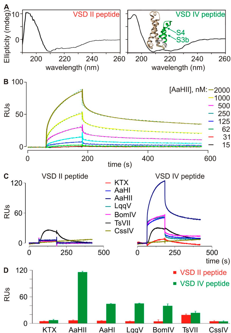
Figure 3. \alpha -Scorpion toxins interact with the isolated rNa v 1.2a VSD IV paddle motif. (A) Shown are the CD spectra of the rNa v 1.2a VSD II and IV paddle peptides used in this paper. Analysis of both spectra revealed the presence of \sim 75\% structured ( \alpha -helix/ \beta -sheet) and \sim 25\% unstructured peptide. Inset shows the crystal structure of the NavAb voltage sensor (3RVY) (Payandeh et al., 2011) in which the paddle motif is indicated in green; wheat shows S1 and S2 helices, and white indicates the portion of S3 and S4 helices outside the paddle. (B) Representative association and dissociation kinetic curves obtained using SPR after the application of varying concentrations of AaHII (15–2,000 nM) over a sensor chip to which 50 fmol of the rNa v 1.2a VSD IV paddle peptide was linked. Toxin was applied after obtaining a steady baseline. Colored traces represent toxin binding obtained after subtraction of the signal from the control flow cell. Green dotted lines depict a fit of the data to a heterogeneous surface ligand model, a typical SPR analysis method (Schuck and Zhao, 2010), which yielded a high affinity K_{D1} of 479 \pm 241 nM ( RU_{max1} = 135 ) and a lower affinity K_{D2} of 747 \pm 203 nM ( RU_{max2} = 23 ; n = 3 ; all results presented as mean \pm SD). The respective contributions of RU_{max1} ( \sim 85\% ) and RU_{max2} ( \sim 15\% ) to the overall RU_{max} (100%) are reminiscent of the percent structured ( \sim 75\% ) versus unstructured ( \sim 25\% ) paddle peptide as observed in the CD spectrum. Toxin concentrations are indicated on the right in a shade of gray corresponding to the sensorgram. (C) Representative SPR traces after the application of 100 nM KTX, AaHI, AaHII, LqqV, BomIV, TsVII, and CssiV over a sensor chip to which the rNa v 1.2a VSD II (left) or IV (right) paddle peptide (500 fmol) was linked. Toxin was applied after obtaining a steady baseline. (D) Binding capacities of 100 nM \alpha -scorpion toxins AaHI, AaHII, LqqV, the \alpha -like scorpion toxin BomIV, and the \beta -scorpion toxins TsVII and CssiV to the VSD II and IV paddle motifs using SPR (error bars represent \pm SEM). Y-axis represents the maximum RUs obtained after toxin application. Note that 500 fmol paddle peptide was used in C and D as opposed to 50 fmol in B. As a result, RUs differ by a factor of \sim 10 .
