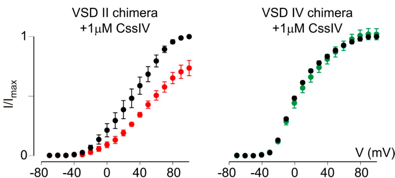
Figure 4. CssIV interacts with the rNa v 1.2a VSD II paddle motif. Shown is the effect of 1 \mu M CssIV on the rNa v 1.2a/K v 2.1 VSD II and IV paddle chimera. Normalized tail current voltage-activation relationships in which the tail current amplitude ( I/I_{\max} ) is plotted against test voltage (V) before (black) and in the presence of toxin (red/green) are displayed. A Boltzmann fit of the obtained data ( n = 3 ; error bars represent mean \pm SEM) reveals a depolarizing shift in V_{1/2} of \sim 14 mV (from 33 \pm 2 mV to 47 \pm 1 mV) for the VSD II chimera, whereas 1 \mu M CssIV does not influence the VSD IV chimera. Holding voltage was -90 mV, and the tail voltage was -60 mV.
