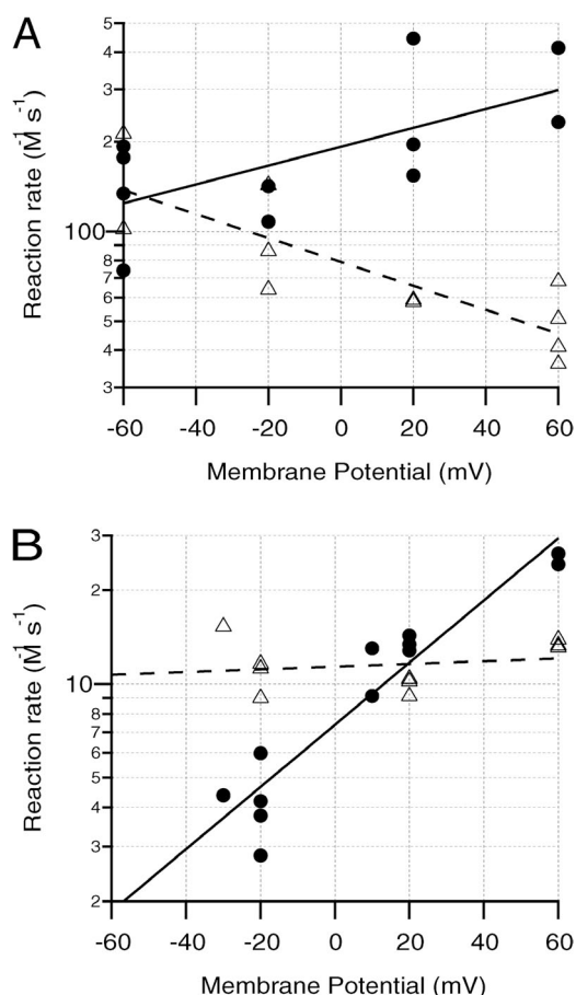
Figure 6. Estimation of MTS-ET reaction rates at 0 mV. (A) S305C. (B) S312C. Each graph is a semilog plot of the second-order rate constant, k , for cis (●) or trans (△) MTS-ET reaction versus voltage. Each data point represents one experiment. Linear fits of \log(k) versus voltage are shown. Interpolating to 0 mV gives k_{\text{cis}}/k_{\text{trans}} \approx 2.4 for S305C and 0.7 for S312C. Solutions were as in Fig. 2, except that for A, the buffers were 30 mM MES, pH 5.3 (cis), versus 50 mM HEPES, pH 7.2 (trans).
