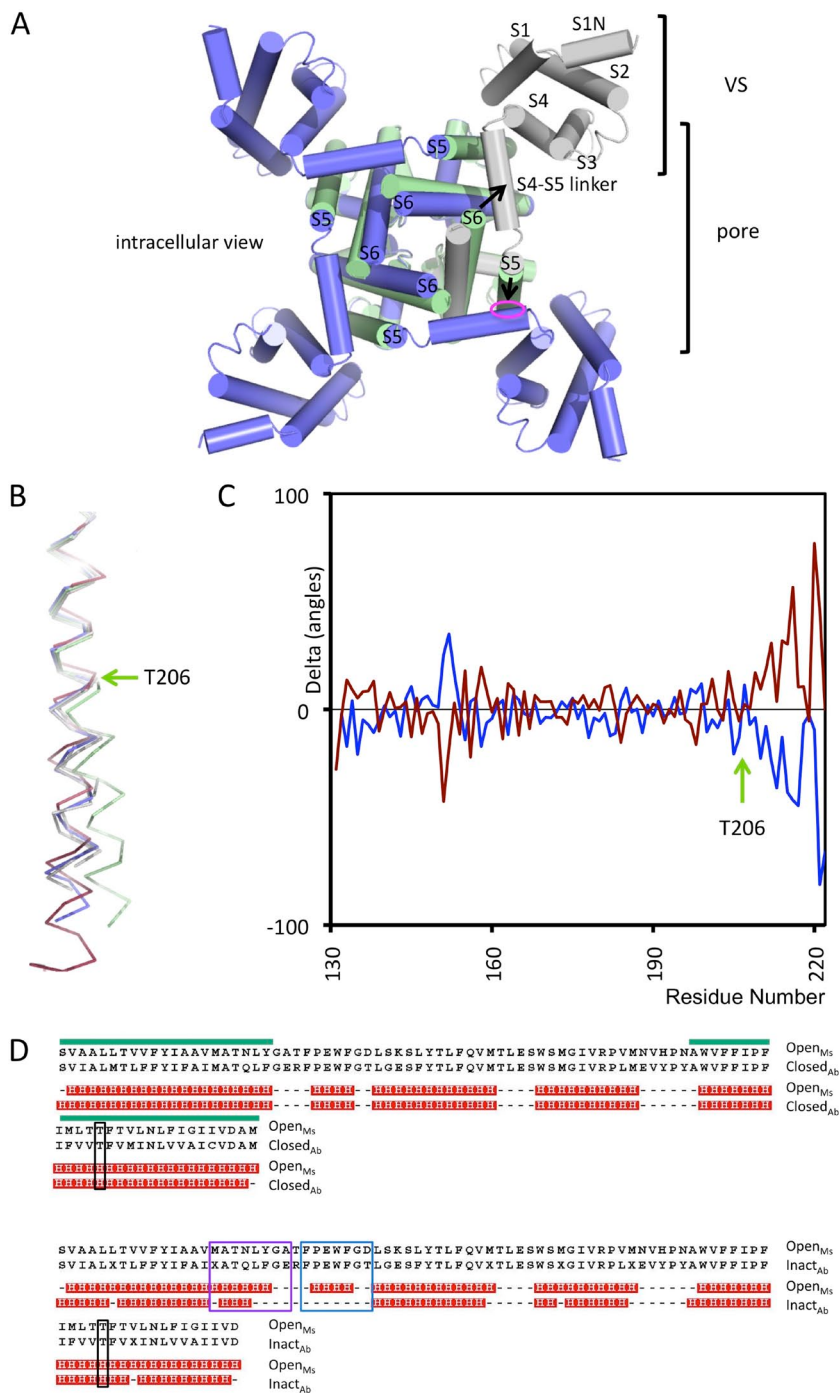
Figure 3. Differences between the open and closed structures. (A) Comparison of the Open Ms (green) pore and the Closed Ab (slate blue) crystal structures, depicted in cylindrical mode viewed from the intracellular surface. The equivalent residue numbers for the pore domain were G129 to M221 in NavMs and G130 to M222 in NavAb. Three-dimensional alignments (in all cases the least-squares superpositions were done using residues 145–198 [or their sequence equivalents] at the top of helices S5 and S6) and figures were made using PyMOL software (Schr  dinger, LLC). The motions associated with the S5 and S6 helices are indicated by the small and large arrows, respectively. One of the Closed Ab monomers is shown in gray, so that it can be seen that the region of the S4–S5 linker that the S5 helix in the open state would impinge on (magenta circle) is in the adjacent, not the same, monomer. (B) The \alpha carbons of the S5 and S6 helices (in stick motif) showing that the Closed Ab (slate blue), Inactivated Ab (gray), and Closed Ac (red) structures overlay closely, but that the Open Ms (green) deviates from the other structures starting at residue T206. (C) Plot of the delta phi (blue) and delta psi (red) angles in the S6 helix as a function of residue number. Values are those of Open Ms structure (PDB accession no. 3ZJZ-A chain) minus those of the Closed Ab structure (3RVY-A chain), demonstrating that the differences start after residue T206 in NavMs and continue to the end of the S6 helix. The single peak at around residue 155 is not related to the transition but simply arises from different interactions of the two proteins, with the different crystallization detergent molecules present adjacent to this site. (D) Secondary structure alignments compared using the 2Struc server (Klose et al., 2010). The position corresponding to the T206 residue in helix S6 is indicated by the black box in both parts. (Top) Open Ms versus Closed Ab . The locations of the S5 and S6 helices are indicated by the horizontal green bars. Both structures have essentially identical secondary structures, even around T206. (Bottom) Open Ms versus Inactivated Ab . The biggest differences are at the top of S5 (purple box) and in the turret loop (cyan box), not in helix S6 nor the region around T206.
