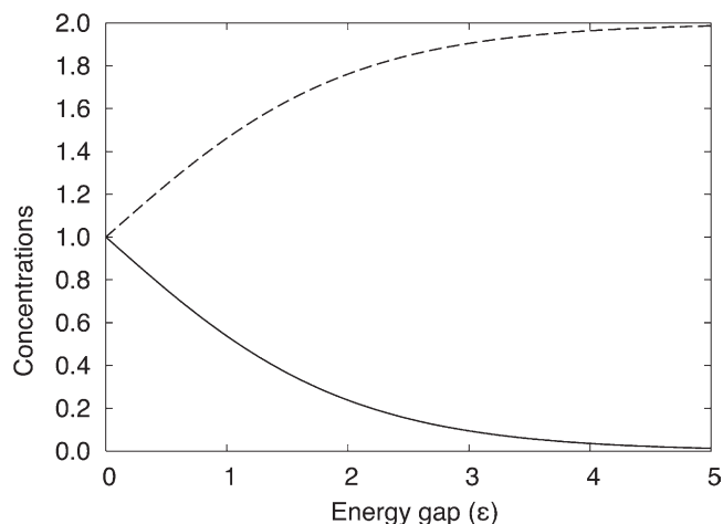
Figure 1. Solute concentrations C_1 (solid line) and C_2 (dashed line) in volumes V_1 and V_2 as a function of the energy gap \varepsilon .
