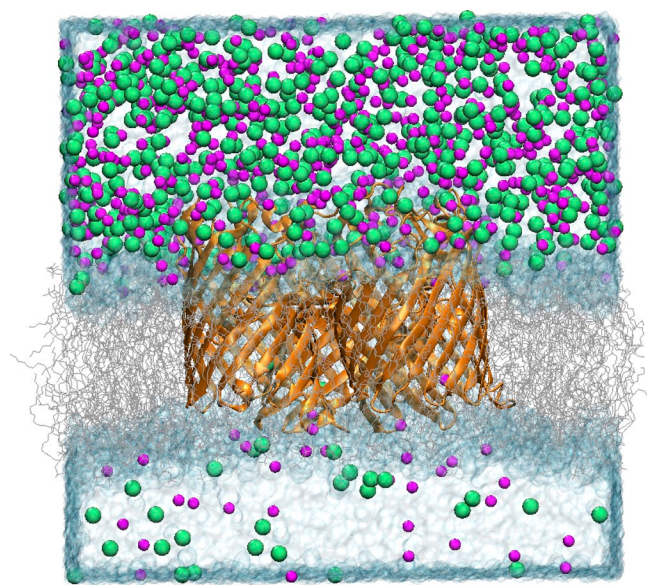
Figure 5. Snapshot of the simulation system consisting of an OmpF trimer embedded in a POPC membrane, fully solvated with 1 M KCl above the membrane and 0.1 M KCl below the membrane, after the application of the energy-step function. \text{K}^+ (magenta) and \text{Cl}^- (green) are shown as spheres.
