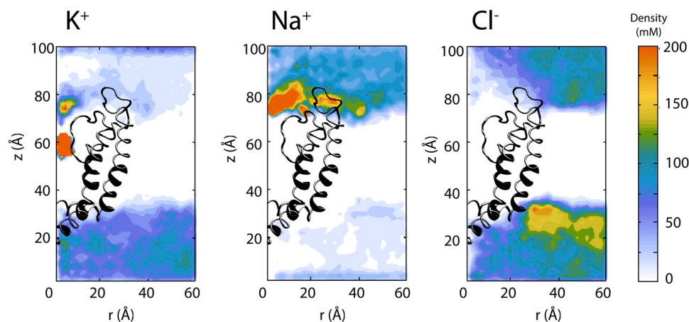
Figure 8. Local density profile of \text{K}^+ , \text{Na}^+ , and \text{Cl}^- ions obtained from the simulations of Kv1.2. Local densities are plotted as a function of radial distance from the pore axis r and the distance from the bottom of the periodic box z .
