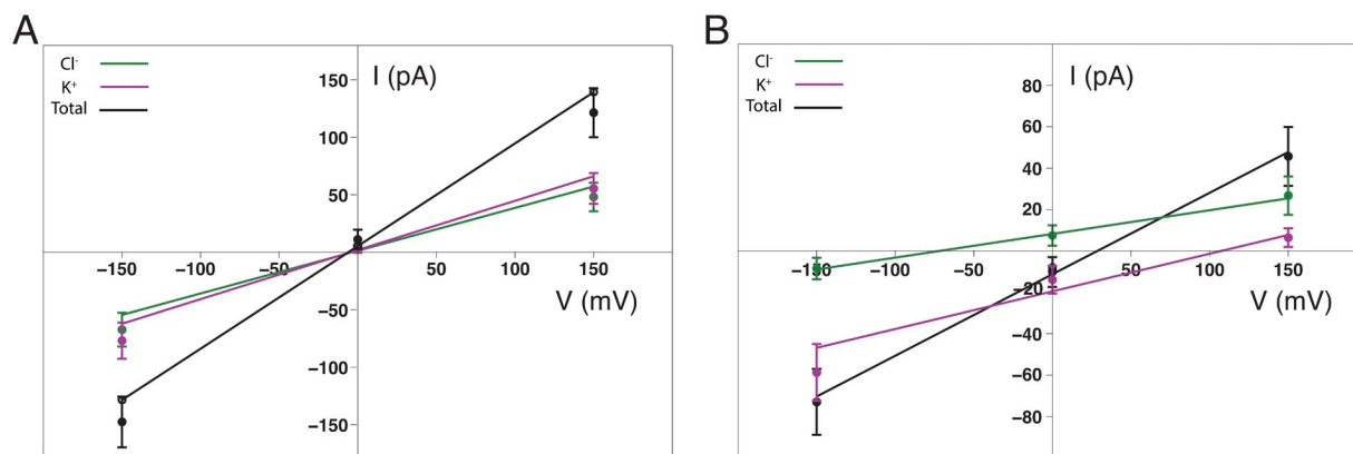
Figure 6. MD simulation of ion permeation and selectivity of OmpF porin. (A) Ion selectivity of OmpF porin. The I-V curves were calculated in (A) 1 M KCl symmetric solution or (B) 0.1:1 M KCl asymmetric solution from MD trajectories. The total current per monomer (black) is the sum of K^+ (purple) and Cl^- (green) currents. Error bars are calculated from Eq. 19.
