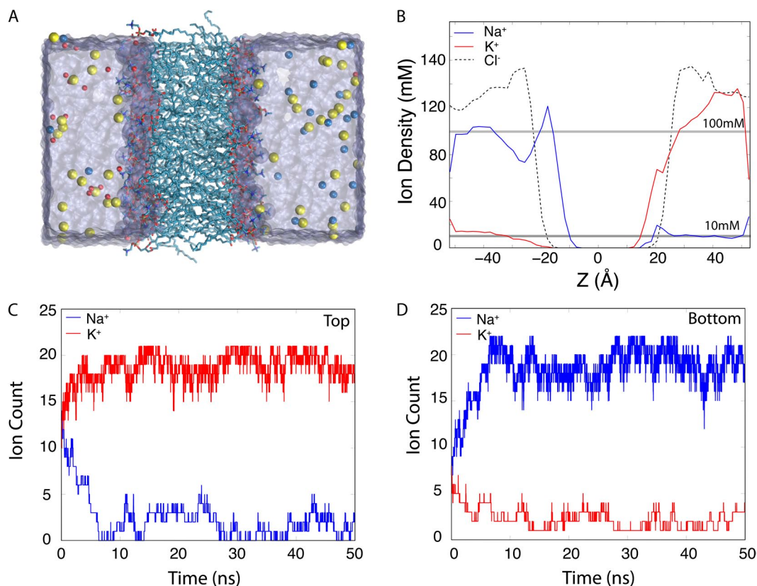
Figure 4. A POPC lipid bilayer simulated under asymmetric ionic concentrations. (A) Snapshot of a POPC lipid bilayer simulated under asymmetric ionic concentrations. Lipid molecules are shown in licorice representation, and Cl^- (yellow), Na^+ (red), and K^+ (blue) ions are shown as spheres. (B) Average density profile of the ions along the z axis normal to the plane of membrane. (C and D) Number of Na^+ and K^+ ions in the top and bottom compartments as a function of time.
