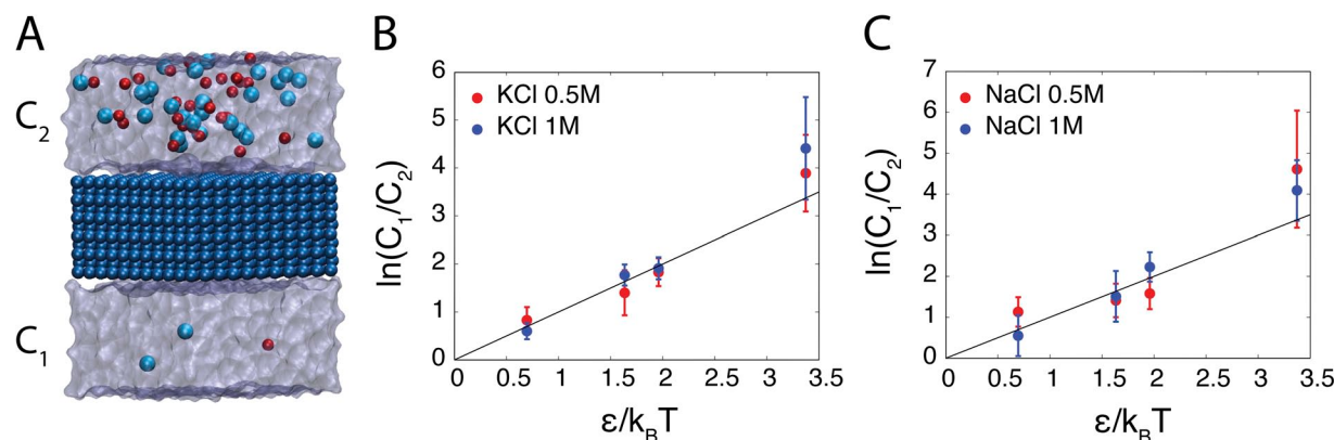
Figure 3. A membrane slab separated by two ionic solutions with concentrations C_1 and C_2 . (A) Snapshot of the simulation system after application of the energy step. (B and C) The ratio of ionic concentration as a function of the applied force for simulations consisting of (B) KCl or (C) NaCl solutions.
