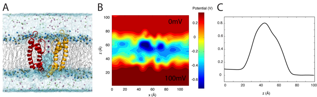
Figure 7. MD simulations of the pore domain of Kv1.2 under physiological conditions. (A) The pore domain of Kv1.2 embedded in a POPC lipid bilayer with asymmetric ionic concentrations. (B) Electrostatic potential map over a cross section of the system normal to the membrane averaged over the last 10 ns of the simulation trajectory. (C) Electrostatic potential normal to the plane of membrane averaged over 1-Å-wide cross sections along the x axis.
