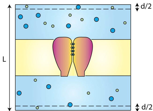
Figure 2. Schematic representation of a typical solvated membrane system. To impose a concentration gradient across the membrane, a constant force is applied to the ions near the boundaries of the periodic box ( z > L_z/2 - d/2 or z < -L_z/2 + d/2 ).
