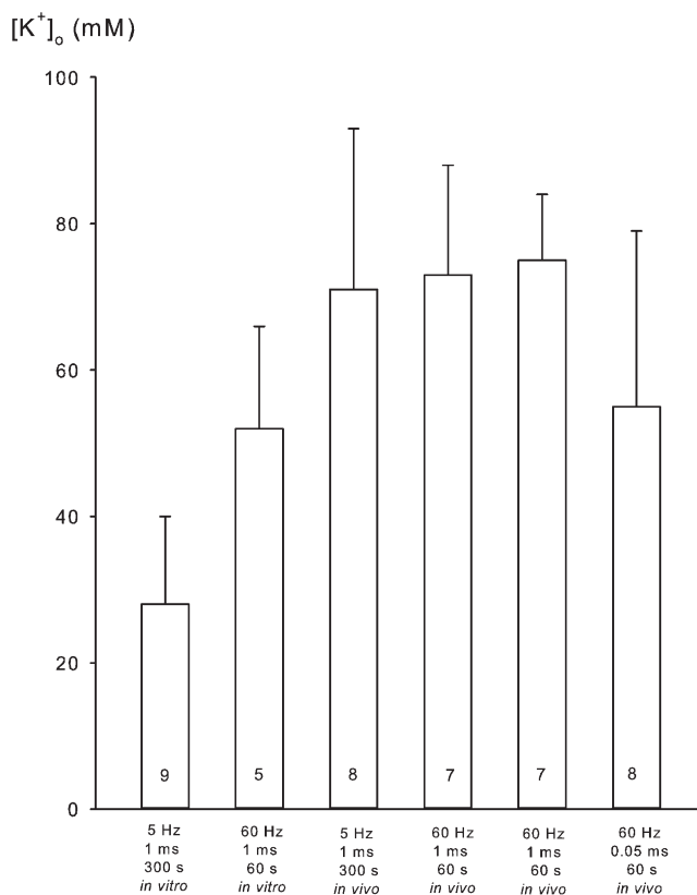
Figure 2. Stimulation-induced expected rise in [\text{K}^+]_o in EDL muscles in six different experiments. Experiments were performed as described in Materials and methods and the legends to Tables 1 and 3. Mean values are obtained by dividing the net loss of \text{K}^+ by the extracellular space measured in the stimulated muscles in vitro (0.194 ml/g wet wt) and in vivo (0.177 ml/g wet wt). Values are given with bars denoting SEM and the number of muscles inside the columns. The frequency and duration of stimulation are given below each column.
