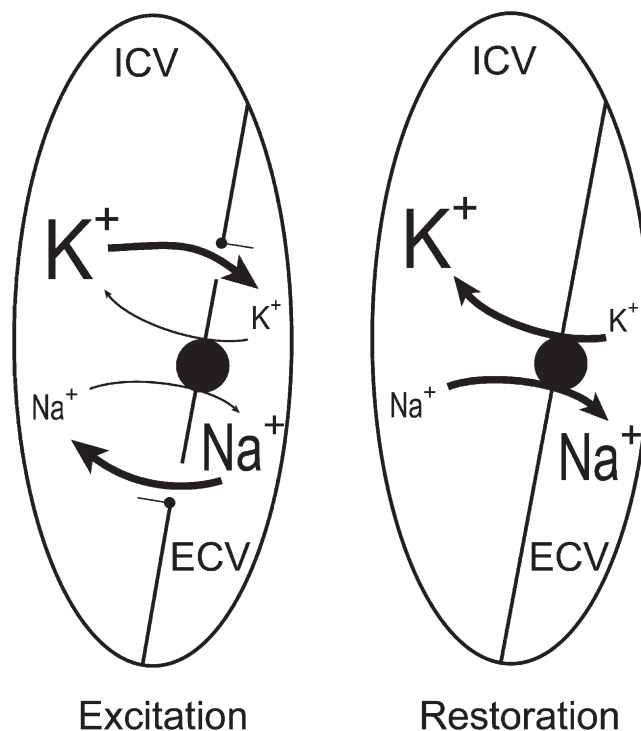
Figure 1. Diagram of excitation-induced exchange of \text{Na}^+ and \text{K}^+ between ECV and ICV. See Table 2. Excitation (left) is induced by a rapid influx of \text{Na}^+ ( 11.2 \mu\text{mol/g wet wt} ) from ECV into ICV, followed by an equivalent efflux of \text{K}^+ ( 11.0 \mu\text{mol/g wet wt} ) from ICV into the ECV. This takes place while the muscles are in air, and during the following washout in ice-cold \text{Na}^+ -free Tris-sucrose, 11 \mu\text{mol/g wet wt} of \text{K}^+ is removed from the ECV as can be seen from the loss of 11 \mu\text{mol/g wet wt} while the \text{Na}^+ taken up into ICV stays in the ICV, leading to a reduction in total \text{K}^+ content and a similar increase in total \text{Na}^+ . As shown in Table 2, the \text{Na}^+ , \text{K}^+ contents are restored during the 600-s incubation without buffer by stimulation of the \text{Na}^+ , \text{K}^+ pumps. When the muscles are incubated in air, these movements of \text{Na}^+ and \text{K}^+ may be followed undisturbed of exchange with a surrounding incubation medium.
