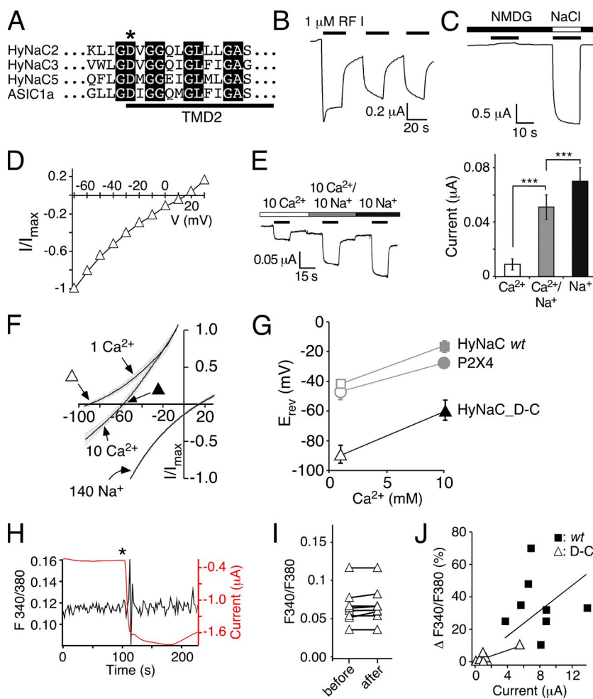
Figure 7. A conserved aspartate is necessary for the high \text{Ca}^{2+} permeability of HyNaC. (A) Alignment of the amino acid sequences of HyNaC2, 3, and 5 and ASIC1a at the beginning of the second transmembrane domain (TMD2) in the one-letter code. The crucial aspartate is indicated by an asterisk. Completely conserved amino acids are shown as white letters on a black background. (B) Representative current trace for HyNaC_D-C activated by 1 \mu\text{M} RFamide I. The amplitude and shape of the transient current component were more variable than for the wt. Mean maximum current amplitudes were 3.45 \pm 1.2 \mu\text{A} for the first activation ( n = 5 ). (C) Representative current trace showing activation of HyNaC_D-C by 1 \mu\text{M} RFamide I in solutions containing 1 mM \text{Ca}^{2+} together with either 140 mM NMDG ^{+} or \text{Na}^{+} . No inward current was visible in NMDG ^{+} solutions. (D) I/V plot for HyNaC_D-C activated by 1 \mu\text{M} RFamide I in standard bath solution. Currents were normalized to the current measured at -70 \text{ mV} , which had an amplitude of -1.1 \pm 0.2 \mu\text{A} ( n = 6 ). (E; left) Representative current trace for HyNaC_D-C in solutions containing 10 mM \text{Ca}^{2+} , 10 mM \text{Ca}^{2+} and 10 mM \text{Na}^{+} , or 10 mM \text{Na}^{+} (nominally free of \text{Ca}^{2+} ). Conditions were as in Fig. 3 B. (Right) Quantitative comparison of current amplitudes. ***, P < 0.001 . (F) I/V relations of HyNaC_D-C in solutions containing 1 or 10 mM \text{CaCl}_2 and no NaCl (which had been replaced by 140 or 126.5 mM NMDG-Cl, respectively) and in a solution containing 140 mM NaCl and 1 mM \text{CaCl}_2 . Lines are the sum of eight to nine individual measurements. SEM is indicated by gray error bars. Experimental conditions were as in
