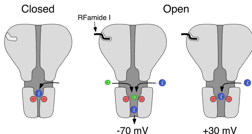
Figure 8. Scheme illustrating \text{Ca}^{2+} permeation through HyNaC. In the closed conformation (left), \text{Ca}^{2+} can probably access the extracellular vestibule through three lateral fenestrations (Jasti et al., 2007; Li et al., 2011) and bind to the conserved aspartates at the outer mouth of the ion pore. After binding of the ligand, HyNaC opens and, at negative membrane potentials, \text{Ca}^{2+} permeates the channel ( -70 mV, middle), liberating the ion pore. At depolarized potentials ( +30 mV, right), however, \text{Ca}^{2+} remains bound to the ring of negative charges and blocks the open pore. Based on the crystal structure of chicken ASIC1 (Jasti et al., 2007).
