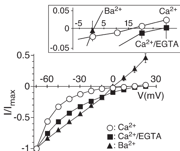
Figure 4. Preventing a rise in [Ca^{2+}]_i changes E_{rev} of sustained peptide-activated currents. I/V relations for HyNaC2/3/5 activated by 1 \mu M Hydra-RFamide I in standard bath (open circles), in standard bath after injection of EGTA (closed squares), and in standard bath in which CaCl_2 had been replaced by BaCl_2 (closed triangles). Currents were normalized to the current measured at -70 mV, which had an amplitude of -4.4 \pm 1.1 \mu A ( Ca^{2+} ), -1.4 \pm 0.2 \mu A ( Ca^{2+}/EGTA ), or -6.0 \pm 0.8 \mu A ( Ba^{2+} ) ( n = 7-8 ), respectively. The inset shows the I/V relations close to the E_{rev} s on an expanded scale.
