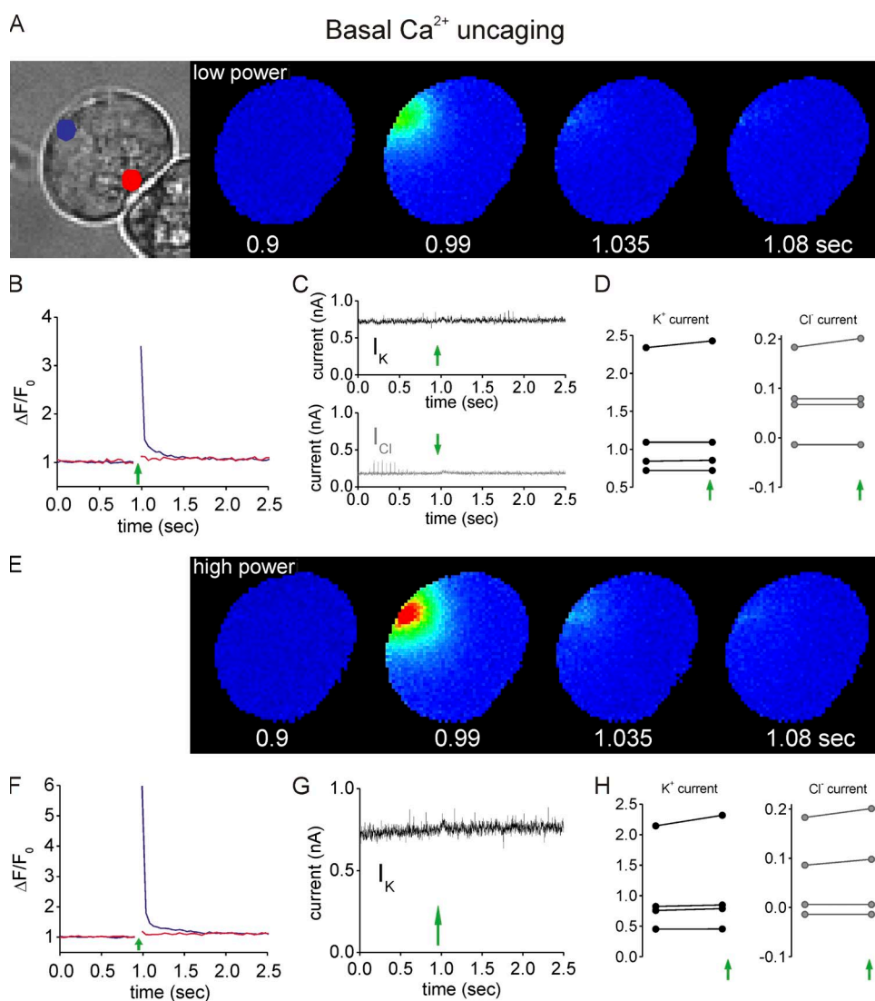
Figure 4. Basolaterally localized increases in [\text{Ca}^{2+}]_i fail to activate \text{K} and \text{Cl} channels. (A) A bright field and pseudocolor image series is shown for a cell in which [\text{Ca}^{2+}]_i was increased under the basal PM (blue dot) using laser parameters identical to Fig. 3. (B) The kinetic demonstrates that a substantial and localized increase in fluorescence was evoked. Increasing the [\text{Ca}^{2+}]_i at the basal PM failed to significantly activate \text{K} channels (C, top) or \text{Cl} channels in TEA- \text{Cl} solution (C, bottom). (D) Paired experiments before and after flash. (E) Similar experiments were performed, but the laser power output was increased to generate a larger increase in [\text{Ca}^{2+}]_i , as shown in E (images) and F (kinetic). (G) Under these conditions, no increase in \text{K}^+ conductance could be evoked. (H) Paired experiments demonstrating that no significant increase in either \text{K}^+ (left) or \text{Cl}^- (right) conductance occurred under these conditions.
