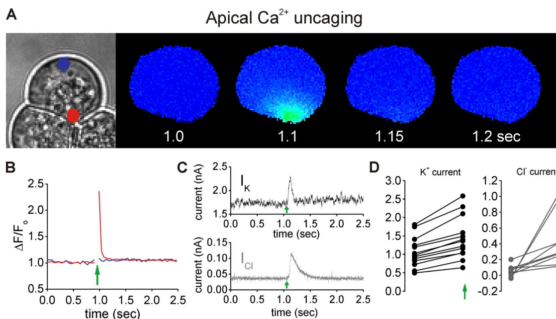
Figure 3. Apically localized increase in [\text{Ca}^{2+}] activates K and Cl channels. Experiments were performed with the buffering conditions established in Fig. 2 (C–F). (A) A bright field and pseudocolored image series in which the [\text{Ca}^{2+}] was increased close to the apical PM (red dot). (B) In these images and kinetic plot, a marked increase in signal was evoked in the apical domain (red line) and remained highly localized. A minimal increase is observed in the basal region (blue line) after laser exposure (green arrow). (C; top) The increase in whole cell \text{K}^+ current evoked by the \text{Ca}^{2+} transient in B is shown. (Bottom) The increase in \text{Cl}^- current after a subsequent apical laser exposure after the bath solution had been exchanged for 140 mM TEA-Cl. A robust increase in whole cell \text{Cl}^- current is evoked. (D) Paired experiments before and after flash.
