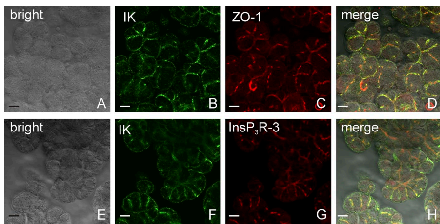
Figure 7. Localization of IK in parotid clumps by immunofluorescence. Immunofluorescence experiments were performed as described in Materials and methods. (A and E) Transmitted laser light images of the parotid clusters. (B and F) The localization of IK is shown and illustrates a prominent PM distribution with enriched localization of channels to the apical domain of the cells. (C) The distribution of the tight junction marker ZO-1 in the clump of cells stained with IK antibodies in B. (G) The localization of InsP_3R-3 , known to localize to the ER juxtaposed to the apical PM, is shown in the same cells. (D) The overlap of IK and ZO-1 is shown. (H) The co-distribution of IK and InsP_3R-3 . Bar, 10 \mu m . Each image is a single z slice acquired at an approximately equatorial plane.
