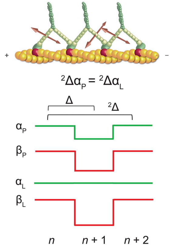
Figure 2. Schematic explanation of ^2\Delta\alpha . The azimuthal changes in probe angle, \alpha_p and lever angle, \alpha_L , over two steps are referred to as ^2\Delta\alpha_p and ^2\Delta\alpha_L , respectively. When walking straight, the probe attached to the myoV lever arm returns to its original orientation every two steps, so that both ^2\Delta\alpha_p and ^2\Delta\alpha_L equal zero and ^2\Delta\alpha_p = ^2\Delta\alpha_L . It can be shown that ^2\Delta\alpha_p = ^2\Delta\alpha_L is a general relationship, regardless of straight walking, so long as \beta_p switches regularly between two states (Section 3 of the Appendix).
