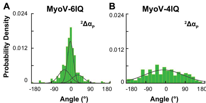
Figure 5. ^2\Delta\alpha_P distributions for myoV-6IQ and myoV-4IQ. Histograms of the ^2\Delta\alpha_P angles were calculated from the mean angles of \alpha_P that were visited during runs of myoV-6IQ (A) and myoV-4IQ (B) and normalized as in Fig. 4. The distributions were fit by a trimodal (6IQ) or a unimodal (4IQ) Gaussian equation; the resulting parameter values are given in Table 2.
