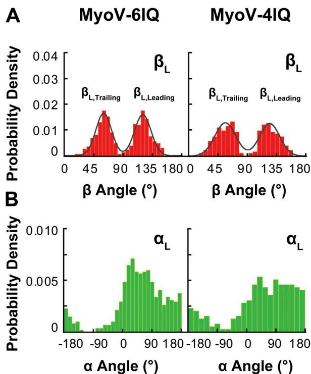
Figure 7. \beta_L and \alpha_L distributions for myoV-6IQ and myoV-4IQ. Histograms of the \beta_L and \alpha_L mean angles visited during individual runs of myoV-6IQ (top: n = 73 molecules and states = 515) and myoV-4IQ (bottom: n = 49 molecules and states = 246). Dwell period selection and normalization as in Fig. 3. (A) \beta_L distributions: Each of these distributions was fit by a bimodal Gaussian equation; the resulting parameters are given in Table 3. (B) \alpha_L distributions.
