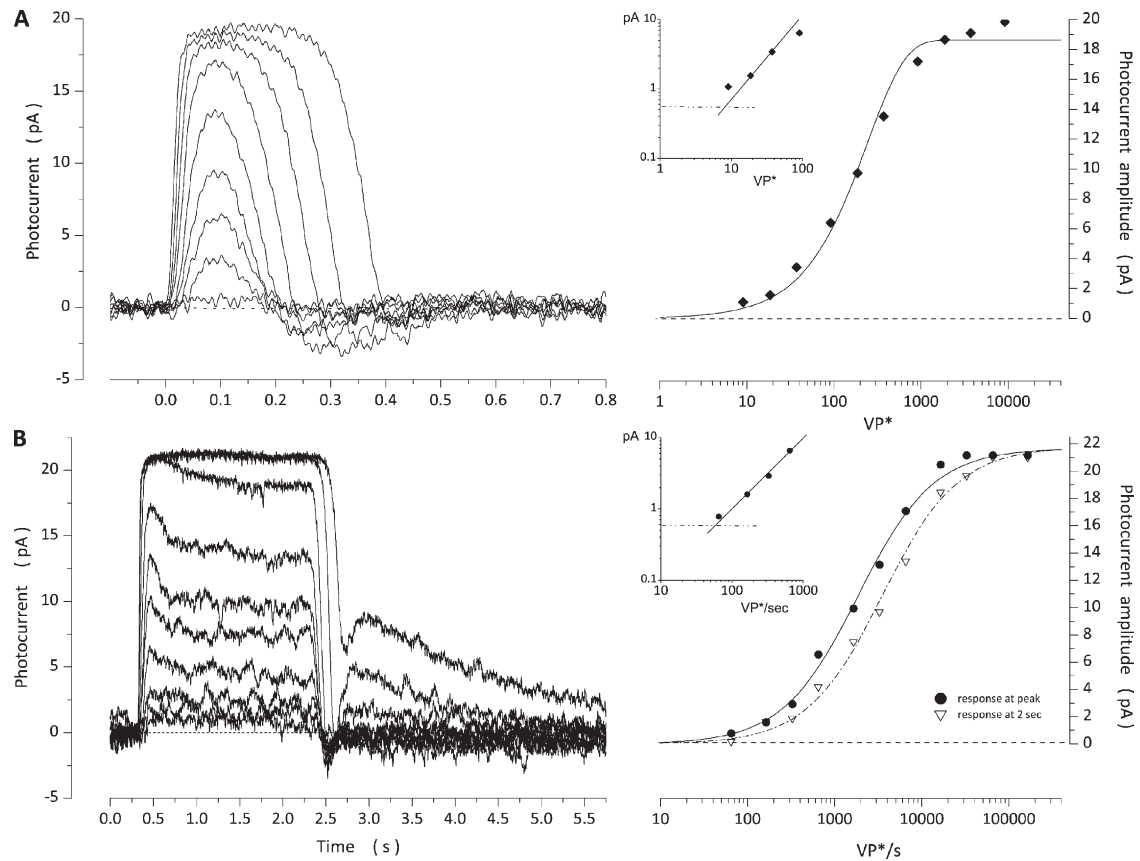
Figure 1. Photocurrents measured under voltage clamp at -40\text{ mV} in a dark-adapted bass single cone in response to 10-msec flashes or 2-s steps of 540\text{-nm} light. (A) Responses elicited with flashes of intensities: 9, 18, 37, 91, 178, 372, 913, 1,933, 3,685, and 9,133 VP^* . Peak amplitude increases with light intensity (right) in a manner well described by an exponential saturation function (Eq. 1.1; continuous line), with I_{peak} = 18.8\text{ pA} and k = 260.1\text{ }VP^* . The inset is a log-log plot to show that signal threshold was \sim 8\text{ }VP^* . (B) Responses elicited with step stimuli of intensities: 65, 327, 651, 1,635, 3,266, 6,513, 16,369, 65,131, and 163,687 VP^*/s . The current at its peak ( \bullet ) is more sensitive to light than in the stationary state ( \nabla ; right). Amplitude dependence on light intensity is well described by a Michaelis-Menten function (Eq. 1.2; continuous line), with I_{peak} = 21.8\text{ pA} and \sigma = 1,844\text{ }VP^*/s for the response at its peak, and I_{max} = 21.8\text{ pA} and \sigma = 3,522\text{ }VP^*/s for the response at 2 s. The inset is a log-log plot of the peak amplitude of the step response to show that signal threshold was 56\text{ }VP^*/s .
