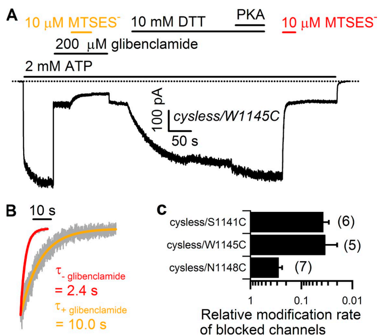
Figure 4. The blocker glibenclamide protects engineered cysteine residues from modification by MTSES - . (A) In an inside-out patch containing thousands of cysless/W1145C -CFTR channels, MTSES - was first (indicated by orange lines) applied in the presence of 200 \mu M glibenclamide (yielding 77% steady-state blockade), and then (red lines) in the absence of glibenclamide after the chemical modification was reversed by the reducing reagent, DTT. (B) Comparison of modification time courses with or without glibenclamide. Portions of the current trace from A were normalized in current amplitude and fitted with single-exponential functions, yielding the modification time constant ( \tau ), as indicated in the figure. This comparison shows that modification rate with glibenclamide (orange) is 24% of that without glibenclamide (red). Thus, the presence of glibenclamide almost completely protects the cysteine against modification, given that the fraction of block is 77%. (C) The bars originating at 1 and ending at a value of <1 on the logarithmic axis correspond to the decrease in the modification rate produced by the blocker glibenclamide. The relative modification rate of blocked channels compared with unblocked ones was corrected for the fraction of block (see Materials and methods).
