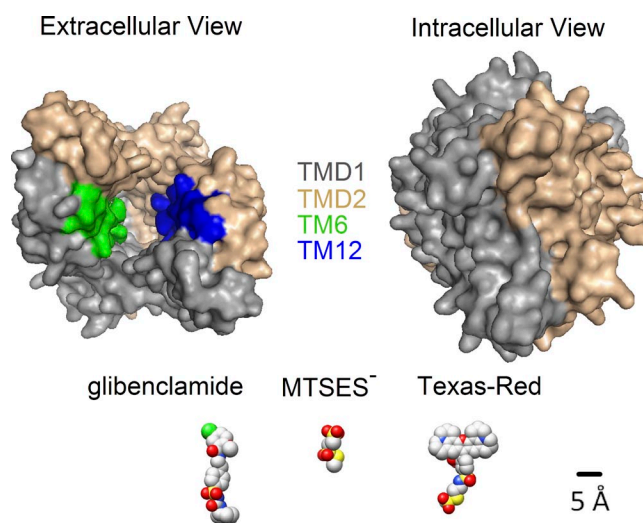
Figure 7. Surface representations of the TMDs (TMD1 and TMD2) of the ABC exporter SAV1866 (Protein Data Bank accession no. 2ONJ), viewed from the extracellular (left) or intracellular (right) side of the membrane. TMD1, TMD2, TM6, and TM12 are colored as indicated. On the same scale (black line), the blocker glibenclamide and two thiol reagents in their most extended configurations were shown for comparison. Note that the structure of the ABC protein shows an obliterated intracellular entrance, but our experimental data suggest that both glibenclamide and MTSES − can readily enter the CFTR pore from the intracellular side when the channel is in the open state.
