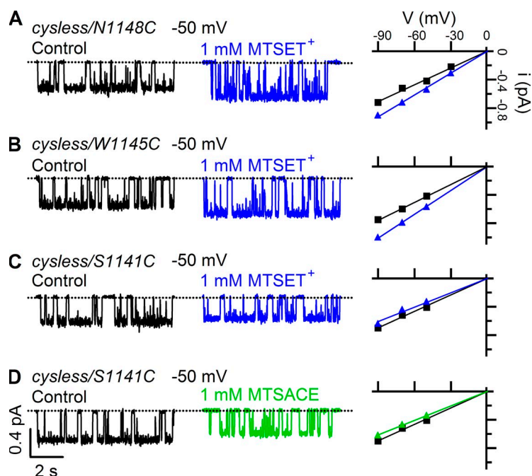
Figure 3. Covalent modifications by MTS reagents alter the single-channel conductance. (A and B) Single-channel recordings at -50 mV show that application of MTSET + increases unitary current amplitudes for cysless/N1148C (A) or cysless/W1145C (B). Linear fits to single-channel current measurements at different voltages yield unitary conductance values for cysless/N1148C (A) of 7.1 pS before (black) and 9.2 pS after (blue) MTSET + treatment, for cysless/W1145C (B) of 7.6 pS before (black) and 10.1 pS after (blue) MTSET + treatment. (C and D) Single-channel recordings show that the unitary current amplitude decreases after MTSET + (C; blue) or MTSACE (D; green) exposure for cysless/S1141C . Linear fits to single-channel current measurements at different voltages yield unitary conductance values for cysless/S1141C of 7.0 pS before (C and D; black) and 6.1 pS after both MTSET + (C; blue) and MTSACE (D; green) treatment. Each data point is the average of three to six patches. Symbols are larger than SEM.
