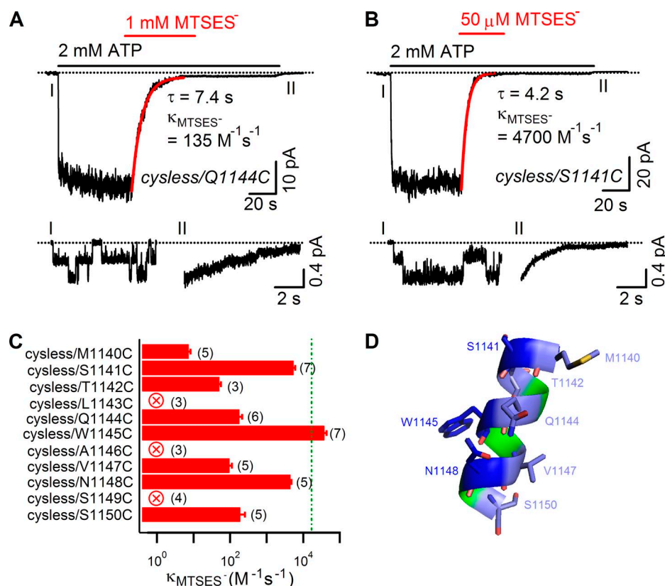
Figure 2. Measurements of the second-order reaction rate reveal that TM12 assumes an \alpha -helical structure. (A and B) Measurements of the second-order reaction rate constant ( k_{\text{MTSES}^-} ) of MTSES - modification in the presence of 2 mM ATP for cysless/Q1144C (A) and cysless/S1141C (B). Single-exponential fitting (red line) of the current relaxation in response to MTSES - treatment yields the modification time constant ( \tau ), the reciprocal of which divided by the concentration of MTSES - gives k_{\text{MTSES}^-} . (Bottom traces I and II) Expanded view of portions of top traces (as marked) to show that the single-channel amplitude is diminished after MTSES - exposure. (C) Summary of the modification rate constant at each position of the cytoplasmic half of TM12. Note that reaction rate at positions 1141, 1145, and 1148 approximates that of MTSES - with free thiols (green line). Crossed circles mark cysteine-substituted channels whose function was not significantly altered by the treatment of MTSES - . The number near each bar represents the number of patches. (D) Helical structure of the cytoplasmic half of TM12 inferred from C. Blue, positions where introduced cysteines were readily accessible to MTSES - ; light blue, positions where cysteines were less accessible; green, positions where no accessibility was observed.
