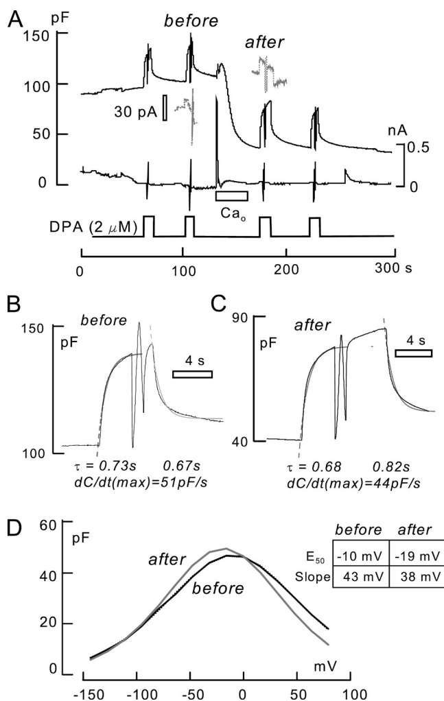
Figure 6. Analysis of DPA-capacitive signals before and after MEND induced by a Ca transient in the presence of 1 mM spermidine and 6 mM ATP. MEND amounts to 68% of C_m . DSF, 4.0. (A) 2 \mu M DPA is applied twice before MEND and twice after MEND for times of 6–10 s. During each application of DPA, voltage is stepped to -150 mV and then ramped to +80 mV to determine the capacitance-voltage relation of DPA. (B and C) Capacitance records indicated by “before” and “after” in A. The magnitudes of DPA-capacitive signal and the time constants of the rising and falling signals (0.67–0.82 s) are not detectably changed. (D) The magnitudes of DPA capacitance-voltage relations are not detectably changed; the peak capacitance undergoes a small 8-mV shift to more negative potentials.
