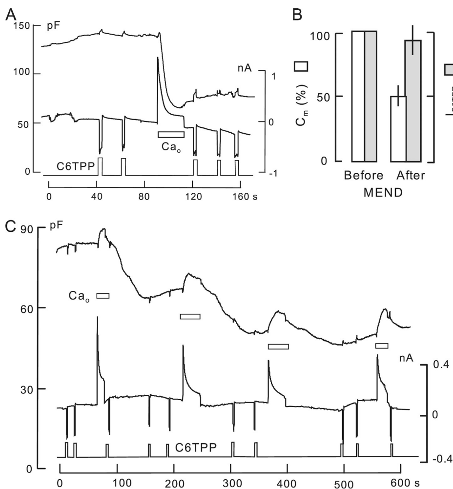
Figure 5. C6TPP currents are nearly unaffected by Ca-induced MEND. 0.3 mM C6TPP is applied briefly multiple times in each experiment, as indicated. (A) 2 mM of the polyamine, EDA, is included in both the cytoplasmic and extracellular solutions to promote rapid MEND (50% in 5 s) during Ca influx by NCX1. Thereafter, C6TPP current is decreased by 12% on average. DSF, 50. (B) Composite results for four experiments similar to A. Ca-activated MEND causes a 50% loss of C_m , whereas C12TPP currents decrease by just 10%. (C) Using a cytoplasmic solution with 6 mM ATP and no polyamine, Ca influx by NCX1 is activated four times. C_m decreases substantially in a delayed fashion after each of the Ca influx episodes, resulting finally in a 45% decrease of C_m . 0.3-mM C6TPP currents are unchanged. DSF, 41.
