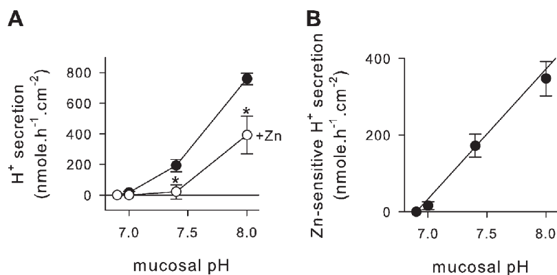
Figure 2. Acid secretion by JME epithelial cultures. (A) Rates of acid secretion in the absence (filled symbols) and presence (open symbols) of 10 \mu M ZnCl_2 . Serosal pH 7.4 and mucosal pH was adjusted to 7, 7.4, and 8; n = 5. *, significantly different from control; t test. (B) Zn-sensitive rates of acid secretion (calculated as the difference from data in A) resulted in an average slope of 339 \pm 33.6\ \text{nmol} \times \text{h}^{-1} \times \text{cm}^{-2} \times \text{pH}^{-1} and a threshold pH of 6.90 (by linear regression).
