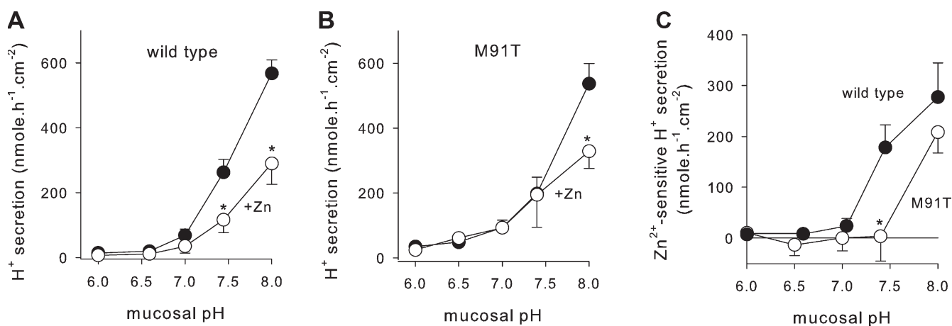
Figure 5. pH dependence of acid secretion of primary human tracheal cultures. Serosal pH 7.4 and mucosal target pH were set to step-wise increasing values over a range of pH 6.0 to 8. (A) Cultures expressing wild-type HVCN1. Filled symbols, untreated; open symbols, 10 \mu M ZnCl_2 mucosally. (B) Primary human tracheal cultures expressing M91T HVCN1. (C) Activation of Zn-sensitive acid secretion by mucosal alkalinization in wild-type (filled symbols) and M91T HVCN1 (open symbols). Data were calculated as the difference of values before-minus-after Zn addition from data in A and B. *, significantly different from control; t test.
