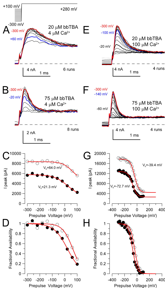
Figure 10. Fractional availability of current in the presence of \text{bbTBA} exhibits voltage independence at negative potentials. (A) \text{Slo1} currents from excised inside-out patches were activated by the indicated voltage protocol (top; prepulse voltages from -300 to +100 mV with 40 -mV increments) with 4 \mu\text{M} of internal \text{Ca}^{2+} and 20 \mu\text{M} \text{bbTBA} . The peak amplitude of the rapidly decaying current exhibits little change until prepulse voltages of 0 mV or more positive. Red trace corresponds to a -300 -mV prepulse and blue to a +60 -mV prepulse. (B) In the same patch, currents were activated with 4 \mu\text{M} \text{Ca}^{2+} along with 75 \mu\text{M} \text{bbTBA} . Red trace, -300 -mV prepulse; blue trace, -20 -mV prepulse. (C) The peak current amplitudes are plotted as a function of prepulse potential for both 20 \mu\text{M} (open circles) and 75 \mu\text{M} (filled circles) \text{bbTBA} . Red lines correspond to fits of a Boltzmann function with V_h = 64.9 \pm 54.4 mV ( z = 0.62 \pm 0.33 e ) and 22.9 \pm 34.9 mV ( z = 0.46 \pm 0.13 e ) for 20 and 75 \mu\text{M} \text{bbTBA} , respectively. (D) Normalized fractional availability was determined based on the fit of the Boltzmann function in C, better illustrating the leftward shift in availability with the increase in \text{bbTBA} . (E) The same protocol was used to activate currents in 100 \mu\text{M} \text{Ca}^{2+} (a different patch) with 20 \mu\text{M} \text{bbTBA} . The peak current at -100 mV (blue trace) shows some reduction compared with -300 mV (red trace). (F) The same patch was exposed to 75 \mu\text{M} \text{bbTBA} , producing more rapid and
