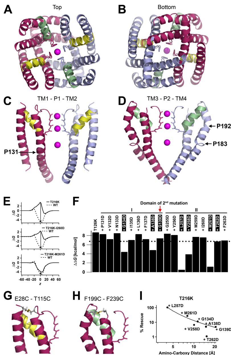
Figure 7. A homology model for \Delta K_{2P}\emptyset channels shows bilateral symmetry with a fourfold symmetric selectivity filter. Model building, refinement, and electrostatic calculations are described in Materials and methods. One subunit is colored in magenta, and the second is colored in blue. The P1 pore helices are in yellow, and P2 pore helices are in green. A file with the main chain coordinates is included in the supplemental material (available at http://www.jgp.org/cgi/content/full/jgp.200910235/DC1 ). (A) The model of K_{2P}\emptyset from the extracellular side reveals overall symmetry like a parallelogram. The model includes residues 1–276 without the TM1-P1 loop (residues 30–91), TM2-TM3 linker (residues 153–173), and TM2-P2 loop (residues 225–238). (B) Model of K_{2P}\emptyset viewed from the cytoplasm. (C) Side view of domain I of both subunits. Pro131 in TM2 is indicated. (D) Side view of domain II of both subunits. Proline residues in TM3 are indicated. (E) Illustration of electrostatic calculations to ascertain the effect of charged mutations on ion permeation (static field contribution). (top) \Delta\Delta G for T216K \Delta K_{2P}\emptyset : \Delta G for the T216K channel (solid line) and \Delta G for the WT channel (dashed line) are shown along the pore axis. The membrane bilayer spans z = -12.5 to z = 12.5 ; \Delta\Delta G = \max[|\Delta G_{T216K} - \Delta G_{WT}|] . This definition of \Delta\Delta G provides a measure of the dominant free energy barrier for ion conduction relative to the WT channel. The arrow indicates where \Delta\Delta G is evaluated. (middle and bottom) Same calculations for T216K-I260D (no rescue) and T216K-M261D (rescue), respectively. (F) Electrostatic \Delta\Delta G (static field contribution) for T216K \Delta K_{2P}\emptyset channels with second site alterations to aspartate (131–139 in TM2 or 255–263 in TM4). Black shading indicates 7 of 18 mutations that restore current. The highest \Delta\Delta G where complementation was observed is marked with a dotted line. The red arrow notes G139D. (G) Section of C showing a disulfide bridge between residues E28C and T115C; the S–S distance in the two subunits ( C_\beta – C_\beta ) are 5.0 and 5.1 Å. (H) Section of D showing a disulfide bridge between residues F199C and F239C; the S–S distance in the two subunits ( C_\beta – C_\beta ) are 6.7 and 6.9 Å. (I) Effectiveness of complementation as a function of distance for T216K \Delta K_{2P}\emptyset channels. Rescue percentage was determined at -100 mV as (I_{Mut} - I_{T216K}) / (I_{WT} - I_{T216K}) . Distances were measured as in Table I. Data were fit to f(x) = a(e^{b/x} - 1) .
