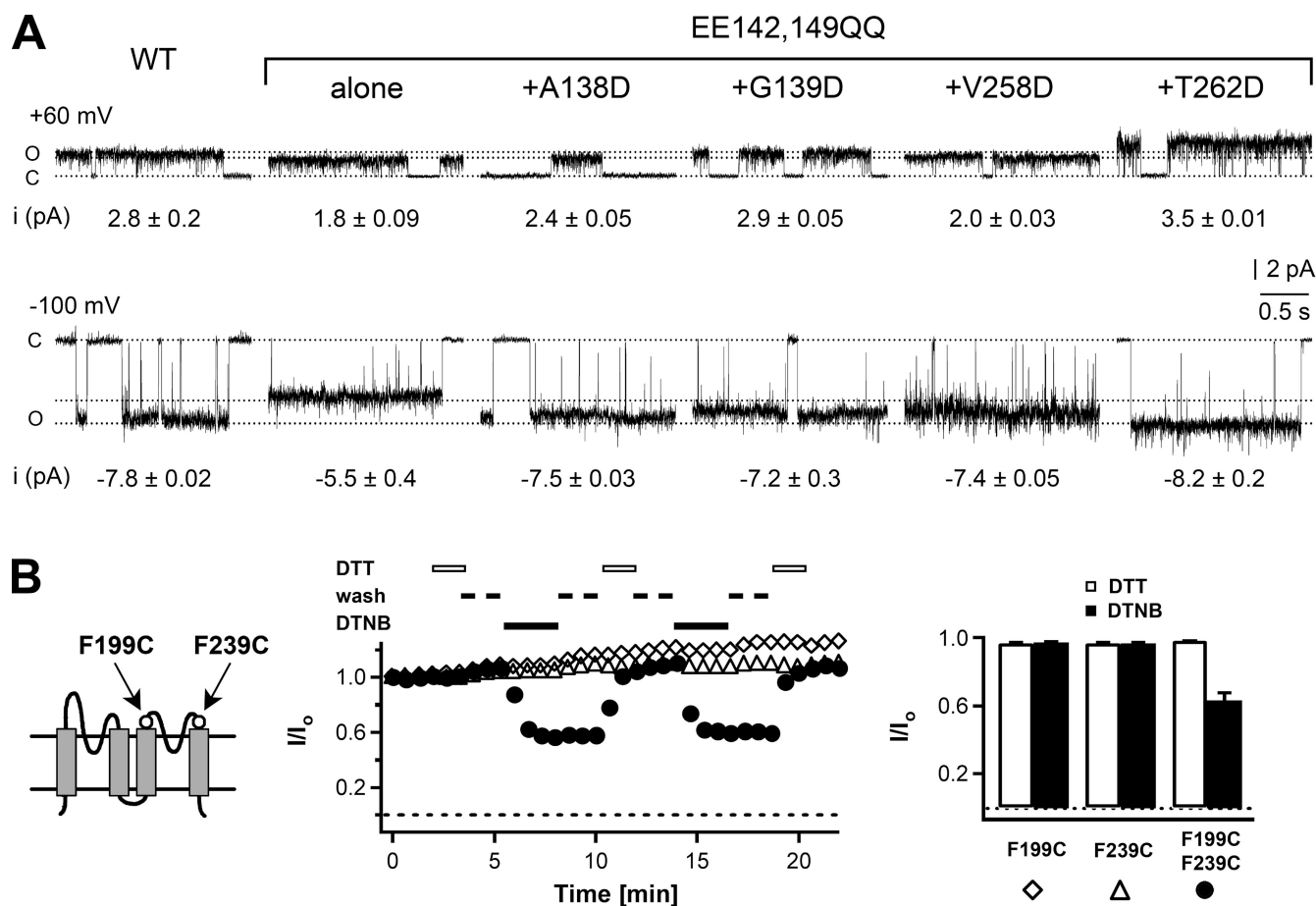
Figure 6. Pore exposure and residue proximity inferred by site effects on single-channel current or disulfide bond formation. (A) Single WT \Delta K_{2p}O channels or EE142,149QQ \Delta K_{2p}O channels with no other change or the indicated third mutation studied at 60 and -100 mV in on-cell patches with 140-mM KCl solution in the bath and pipette (see Materials and methods). Unitary currents (i) were determined from 2 to 8.5 min of recording from two to six patches sampled at 20 kHz, filtered at 5 kHz with one to nine channels per patch (median = 2), and noted \pm SEM. Exemplar currents were filtered at 500 Hz. Open (O) and closed (C) levels are indicated. (B, left) Predicted topology of \Delta K_{2p}O indicating the location of F199 and F239. (middle) Whole cell currents studied at 30 mV. The channels studied had the native external cysteine in the first external loop altered to serine (C73S). Application of 0.5 mM DTNB reduces C73S F199C F239C \Delta K_{2p}O current (black circles), and 5 mM DTT reverses the effect. Current of \Delta K_{2p}O C73S F199C (open diamonds) or C73S F239C \Delta K_{2p}O (open triangles) is not affected by exposure to DTT or DTNB. Plot is normalized current for single cells; every 20th data point. (right) Current \pm SEM at 30 mV after application of 5 mM DTT (open bars) or 0.5 mM DTNB (closed bars) normalized to the amplitude of the same cell without treatment for \Delta K_{2p}O channels with the following changes: C73S and F199C; C73S and F239C; C73S and F199C and F239C ( n = 2-4 cells).
