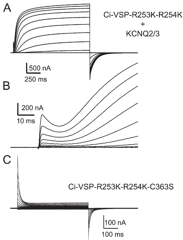
Figure 6. (A) The ionic current through KCNQ2/3 was not decreased after depolarization when coexpressed with the mutant R253K-R254K. (B) Ci-VSP is shown to be expressed because its sensing currents can be observed immediately after depolarization. (C) The phosphatase-inactivated mutant R253K-R254K-C363S was expressed alone to study sensing currents. The R253K-R254K-C363S mutant exhibits ON sensing currents that look very similar to those observed from the C363S mutant, although the OFF currents did not display the typical change in mode, observed with the C363S mutant (see Fig. 3). Pulses range from -100 to +100 mV. HP = -90 mV for ionic currents and -60 mV for sensing currents.
