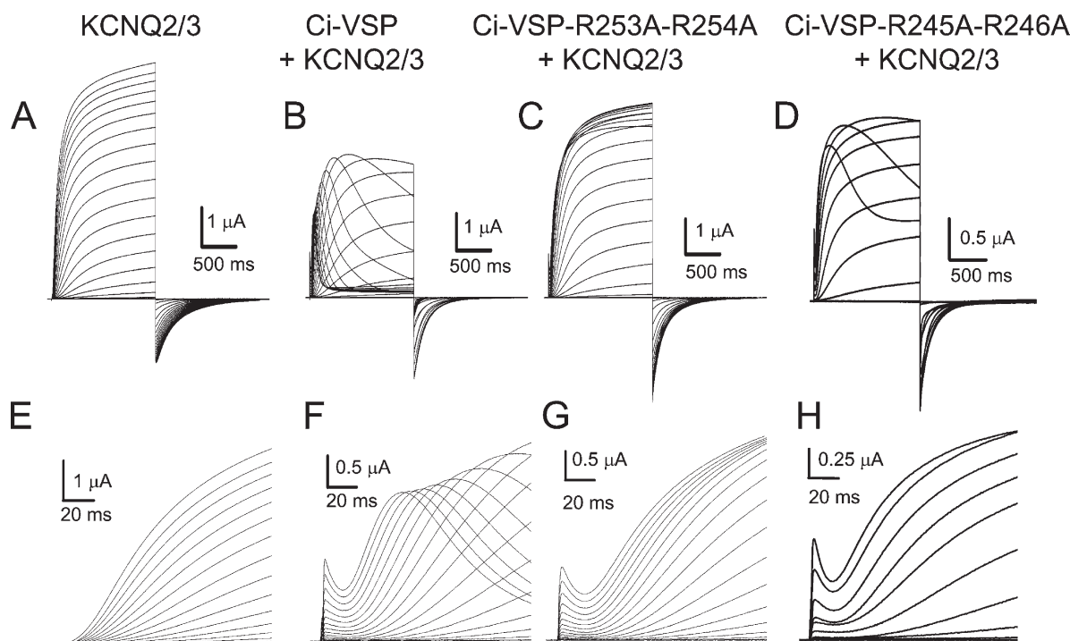
Figure 4. Phosphatase activity of Ci-VSP monitored by the activity of the potassium-selective, voltage-, and PI(4,5)P 2 -dependent channels KCNQ2 and KCNQ3. (A) Currents of KCNQ2/3 expressed without Ci-VSP. (B) When KCNQ2/3 were expressed with the WT form of Ci-VSP, a strong decrease in the activity was observed at potentials above +20 mV. (C) Coexpression with the mutant R253A-R254A caused a slight decrease in the current of KCNQ2/3, only observable at very positive potentials. (D) Likewise, coexpression with the mutant R245A-R246A caused an initial decrease in the current of the channels at potentials above +80 mV. However, the effect on the ionic current was less profound than that observed with the mutant R253A-R254A. (E) Transient initial currents were not observed when mRNA coding for Ci-VSP was not injected in the oocytes along with the mRNA for KCNQ2/3. (F–H) In contrast, transient initial currents were observed in the presence of the phosphatase. These currents are the sensing currents of Ci-VSP. Pulses range from −100 to +100 mV. HP = −90 mV. For A–C and E–G, the interval between pulses was 10 mV. For D and H, it was 20 mV.
