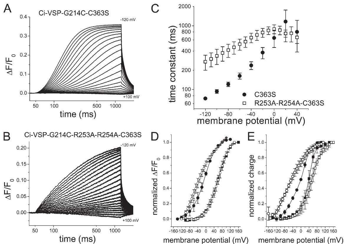
Figure 8. The mutants G214C-C363S and G214C-R253A-R254A-C363S were expressed in oocytes and labeled with TMRM. Changes in the fluorescence emission of TMRM observed from the mutant G214C-R253A-R254A-C363S (B) were slower than those observed from the mutant G214C-C363S (A) when a conditioning pulse to +80 mV was applied for 5 s to produce the relaxation of the VSD. The differences in the time constant of the fluorescence were significant for all the potentials tested below -10 mV (C), reaching up to fourfold below -100 mV. The voltage dependence of the normalized amplitude of the fluorescence change showed no difference between G214C-C363S (D; filled squares) and G214C-R253A-R254A-C363S (D; open squares) when the HP = -60 mV. However, the amplitude of the fluorescence change from the G214C-R253A-R254A-C363S mutant showed a clear shift toward negative potentials (D; open circles) with respect to the G214C-C363S mutant (D; filled circles) when the membrane was conditioned to +80 mV for 5 s. Likewise, the voltage dependence of the charge movement displays a small shift toward positive potentials for the mutant G214C-R253A-R254A-C363S (E; open squares) with respect to the mutant G214C-C363S (E; filled squares). Prepulsing the membrane to +80 mV for 5 s produces a deeper relaxation of the VSD of the mutant G214C-R253A-R254A-C363S, as reflected by a larger shift toward negative potentials (E; open circles) with respect to the shift observed in the mutant G214C-C363S (E; filled circles).
