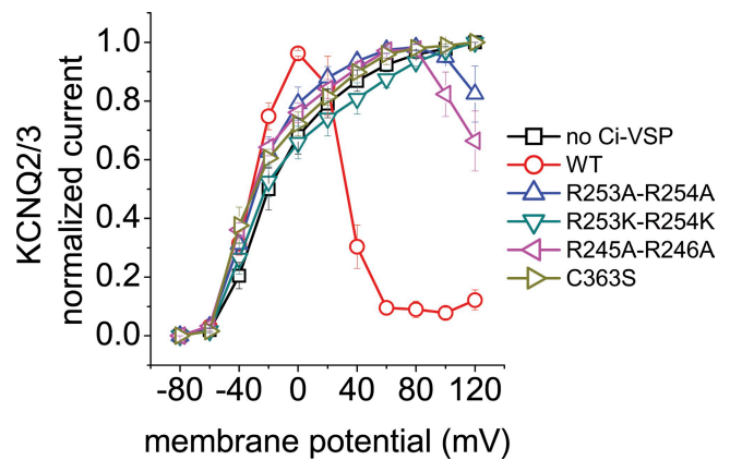
Figure 7. The activity of the Ci-VSP expressed as the average of the amplitude of the KCNQ2/3 current after 1.5 s of depolarization normalized to the maximum current. When compared with the C363S mutant, the only values significantly different are those from the R253A-R254A-C363S mutant and the R245A-R246A mutant for potentials above +100 and +80 mV, respectively.
