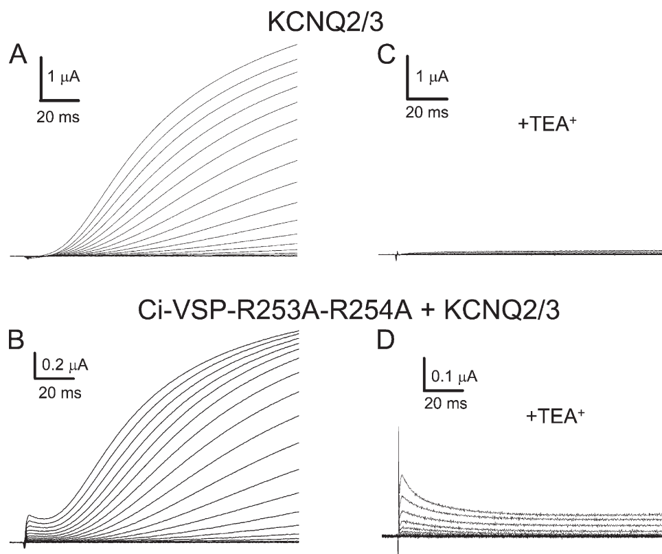
Figure 5. Block of ionic current from oocytes expressing KCNQ2/3 alone (A and C) and coexpressed with Ci-VSP R253A-R254A (B and D). (A) The K^+ currents of KCNQ2/3 when depolarizing the oocytes. (B) Coexpression of the mutant R253A-R254A and KCNQ2/3 yielded K^+ currents and, in addition, sensing currents from Ci-VSP. (C) Oocyte expressing KCQ2/3 alone shows no currents after replacing K^+ for TEA^+ in the internal and external solutions during cut-open recording. (D) In contrast, when KCNQ2/3 was coexpressed with the R253A-R254A mutant of Ci-VSP, TEA treatment showed the transient current characteristic of the sensing currents of Ci-VSP. Pulses range from -100 to +100 mV. HP = -90 mV.
