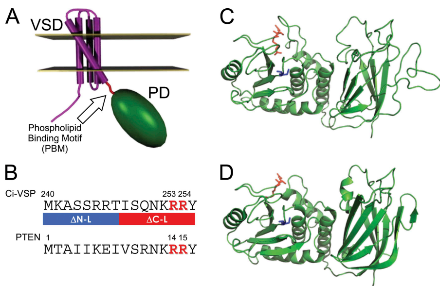
Figure 1. (A) Cartoon representation of the structure of Ci-VSP. The N terminus of Ci-VSP spans four transmembrane segments forming the VSD, and the fourth segment (S4 segment) of the VSD is connected to the PD by the PBM. (B) The proposed PBM of Ci-VSP shares 50% identity with the first 16 amino acids of the PTEN. (C) Homology model of the PD of Ci-VSP. This homology model was created by the online package 3D-jigsaw using residues 240–576 of Ci-VSP ( http://bmm.cancerresearchuk.org/~3djigsaw/ ). The obtained model comprises residues 253–574. (D) Crystal structure of PTEN. The crystal structure of PTEN is constituted by residues 14–351 (Lee et al., 1999). Arginines 253 and 254 of Ci-VSP (C) and 14 and 15 of PTEN (D) are displayed in red. These residues are implicated in the formation of the putative PBM in these proteins. Cysteine 363 of Ci-VSP and 124 in PTEN are displayed in blue. These residues are essential for the activity of the catalytic site.
