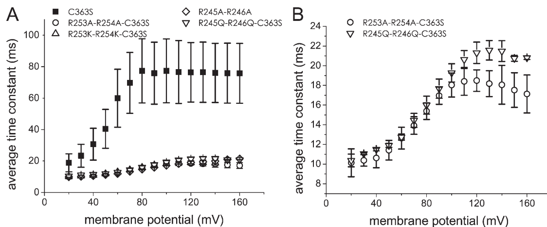
Figure 3. Average time constant of the OFF sensing current of different mutants of Ci-VSP. (A) The OFF sensing current recorded from the PBM mutants (open symbols) R253A-R254A-C363S ( n = 5 ), R253K-R254K-C363S ( n = 4 ), R245Q-R246Q-C363S ( n = 4 ), and R245A-R246A ( n = 4 ) were significantly faster than those recorded from the C363S mutant (filled squares; n = 5 ) for all potentials tested above +20 mV (HP = -60 mV). (B) The mutant R245Q-R246Q C363S displayed slower OFF sensing current than those from the mutant R253A-R254A-C363S for pulses above +100 mV.
