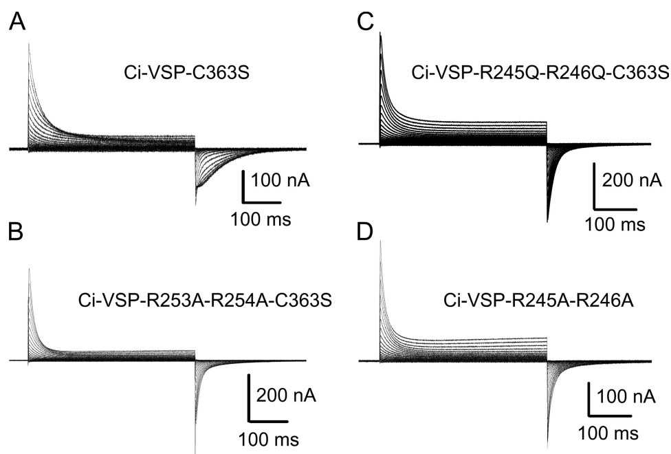
Figure 2. Sensing currents from oocytes expressing different mutants of Ci-VSP. Sensing currents were recorded by applying voltage pulses of 400 ms, ranging from -100 to 140 mV. The HP was -60 mV. (A) Sensing currents for the phosphatase-inactivated mutant Ci-VSP C363S. When pulsing to positive potentials from the HP, all the mutants, R253A-R254A-C363S (B), R245Q-R246Q-C363S (C), and R245A-R246A (D), displayed sensing currents similar to those observed with the mutant C363S. In contrast, during the repolarization to the HP, all the PBM mutants displayed faster OFF sensing currents.
