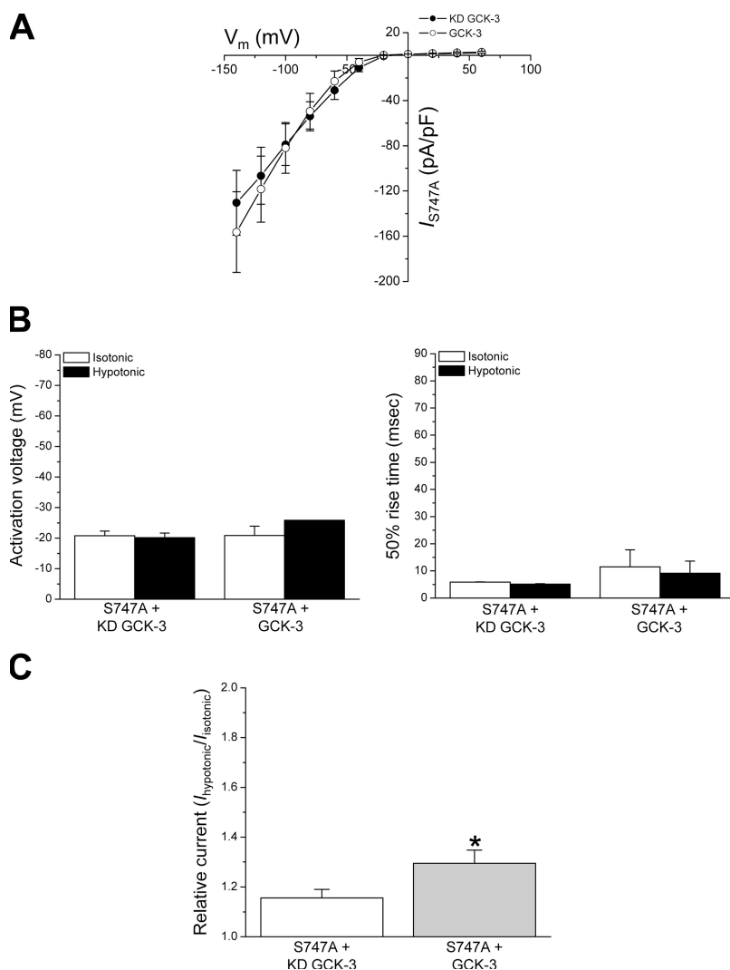
Figure 4. Mutation of S747 to alanine prevents GCK-3-mediated inhibition of CLH-3b. (A) Current-voltage relationships of the S747A mutant coexpressed with functional or KD GCK-3. Values are means \pm SE ( n = 6-9 ). (B) Activation voltages and 50% rise times of whole cell currents in cells coexpressing the S747A mutant and KD GCK-3 or GCK-3. Values are means \pm SE ( n = 6-9 ). (C) Effect of cell swelling on current amplitude in cells coexpressing the S747A mutant and KD GCK-3 or GCK-3. Values are means \pm SE ( n = 6-9 ). *, P < 0.04 . Data were obtained as described in the legend to Fig. 1.
