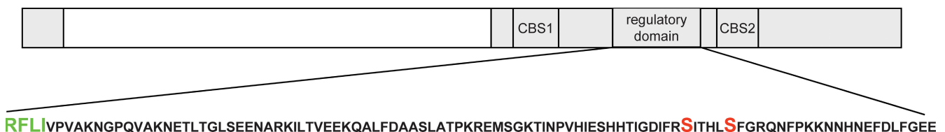
Figure 2. CLH-3b functional domains. Open and shaded bars are predicted intramembrane and intracellular domains, respectively. Relative size of domains is approximately to scale. The regulatory domain is a 101-amino acid splice insert unique to CLH-3b (Denton et al., 2004). Sequence of regulatory domain is shown. Green highlighting indicates location of GCK-3 binding site (Denton et al., 2005). Serines 742 and 747 are highlighted in red.
