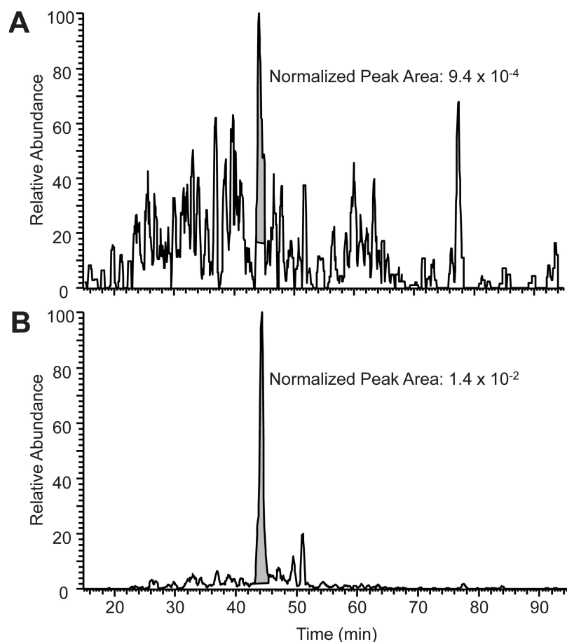
Figure 3. Representative extracted ion chromatograms from targeted MS/MS analysis of the SITHLSFGR peptide phosphorylated at both S742 and S747 in cells expressing KD GCK-3 (A) or functional GCK-3 (B). Shading shows the peak areas for the doubly phosphorylated SITHLSFGR peptide. These areas were normalized to the CLH-3b tryptic peptide KILTVEEK and are reported on each plot. In cells expressing functional GCK-3, phosphorylation of SITHLSFGR increases 15-fold. Similar fold changes were obtained in three replicate analyses and with normalization of the peak areas to two other CHL-3b tryptic peptides, LVHGSSGGIFENESR and YVDSQIGTK.
