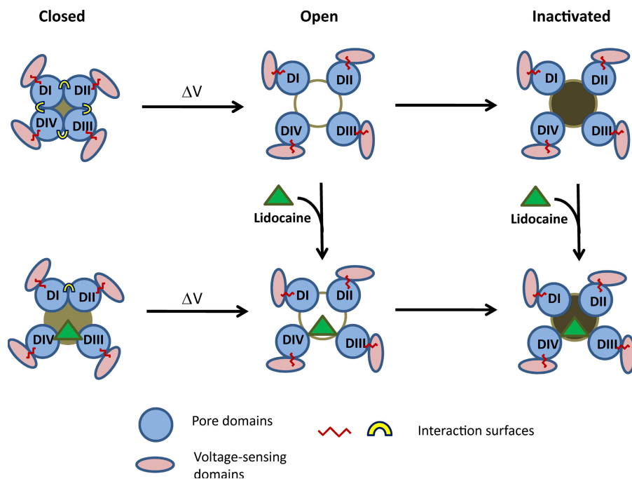
Figure 9. A schematic depicting a preliminary model of sodium channel modulation by local anesthetics. Local anesthetic binding to the open and inactivated state primarily stabilizes the pore segments of domain III and to some extent of domain IV in the open state. Because the movement of pore helices (blue circles) is coupled to the voltage sensor (pink ellipsoids), local anesthetic binding also stabilizes the voltage sensors of domains III and IV in the activated state. The interdomain interaction is mediated by the residues near the inner helix bundle crossing. In this model, as in the potassium channel, these residues interact in the closed state of the channel. This interaction is disrupted if the local anesthetic acts as a wedge and prevents the S6 segments of domains III and IV from fully closing.
