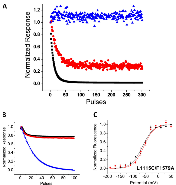
Blue symbols represent the current in the presence of QX-314 in the L1115C channel, obtained with the same protocol pulse. (B) Effect of QX-314 on the voltage-dependent fluorescence of the L1115C/F1579A mutant channel. F-V relationships from TMR-labeled L1115C/F1579A mutants before (black) and after (red) a 3-mM QX-314 application (after 100 depolarizing pulses at 10 Hz frequency). These fluorescence intensity changes were normalized to the maximum fluorescence change. Circles represent the means \pm SE of four independent experiments, and the line represents the best fit of the averaged data to a single Boltzmann function.
