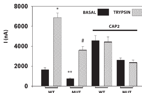
Figure 6. Amiloride-sensitive I_{Na} of triple mutant α-K561A, β-R503A, and γ-R515A channels activated by CAP2. WT α-, β-, γ-, or mutant α-K561A, β-R503A, and γ-R515A ENaC cRNA (0.3 ng each) and 1 ng CAP2 cRNA were injected into oocytes. 24 h after injection, two-electrode voltage clamp assays were conducted. Currents measured in the presence and absence of 10 μM amiloride, while clamping the membrane voltage to -100 mV, were digitized and recorded. Batches of oocytes were extracted from four different frogs ( n = 24 ). Results are expressed as the means \pm SE. Statistical significance was determined using an unpaired Student's t test. Basal WT I_{Na} versus WT trypsin-stimulated I_{Na} : *, P < 0.0001 ; basal WT I_{Na} versus basal triple mutant I_{Na} : **, P < 0.0011 ; basal triple mutant I_{Na} versus triple mutant trypsin-stimulated I_{Na} : #, significant P < 0.0001 .
