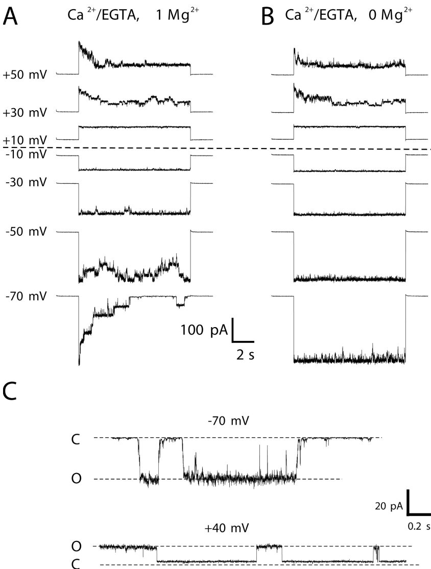
Figure 2. Divalent cations selectively affect gating of Cx46 hemichannels at negative membrane potentials. (A and B) Multichannel cell-attached patch recordings from a Cx46-expressing oocyte recorded with (A) 1 mM \text{Mg}^{2+} present in the patch pipette and (B) no added \text{Mg}^{2+} in the patch pipette. In both cases, \text{Ca}^{2+} was buffered to very low levels with EGTA (Materials and methods). Shown are currents in response to 10-s voltage steps from -70 and +50 mV applied in 20-mV increments. No endogenous channel activity was present these patches. In the presence of 1 mM external \text{Mg}^{2+} , Cx46 hemichannels essentially remained open at modest voltages (see traces at -10 and +10 mV) and tended to close for either polarity of membrane voltages. Hyperpolarization led to full and robust closure (see trace at -70 mV), whereas depolarization left a residual current (see current trace at +50 mV). The current records were leak subtracted as described in the Materials and methods. When there was no added external \text{Mg}^{2+} , gating at positive voltages did not change, whereas gating at negative voltages changed significantly. In the example shown, gating was essentially abolished at hyperpolarizing voltages up to -70 mV. (C) Cell-attached patch recordings of single Cx46 hemichannels highlighting the two different types of gating at negative ( -70 mV) and positive ( +40 mV) voltages, termed loop gating and V_j gating, respectively. Recordings were obtained with standard IPS (containing 1 mM \text{Mg}^{2+} ). Loop gating is characterized by gating transitions between fully closed (C) and open (O) states (left), whereas V_j gating transitions occur between the open state (O) and a long-lasting subconductance state (right). Currents were leak subtracted as described in Materials and methods. All currents were filtered at 1 kHz and data were acquired at 5 kHz.
