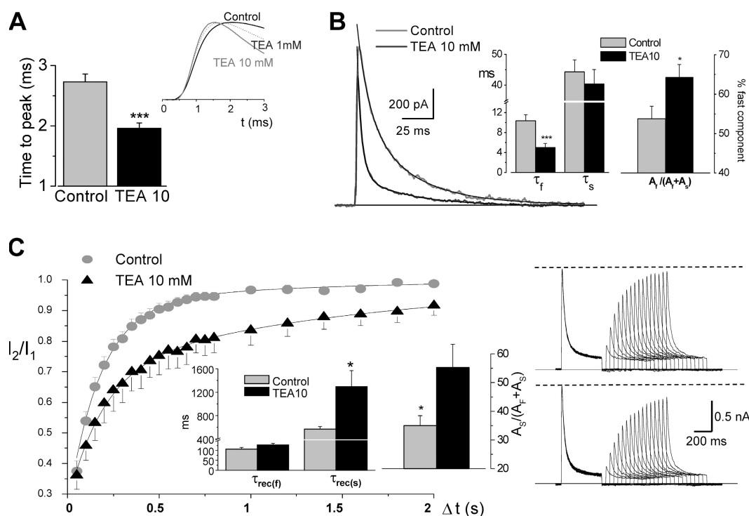
Figure 6. Modulation by TEA of the kinetics of Kv4.3+DPPX channels. (A) Speed of activation was studied in depolarizing pulses to +40 mV in outside-out macropatches, and was calculated as the time to peak current amplitude. The traces in the figure show normalized currents obtained in one representative cell in control (black line) and in the presence of 1 mM TEA (dotted line) and 10 mM TEA (gray line). The bar plot shows the mean data from 15 patches in control and in the presence of 10 mM TEA. ***, P < 0.001 for paired data. (B) The time course of inactivation of the current elicited in 200-ms depolarizing pulses to +40 mV was fitted to a biexponential function both in control and in the presence of TEA (10 mM). The figure shows two representative traces from a macropatch together with their corresponding fits. The bar graphs display the inactivation time constants ( \tau_s and \tau_f ) and the relative amplitude of the fast component obtained in control and in the presence of 10 mM TEA. Mean \pm SEM of 14 cells. *, P < 0.05 ; ***, P < 0.001 for paired data. (C) Recovery from inactivation at -80 mV in the presence of 10 mM TEA determined with the same double pulse protocol described in Fig. 3 D. The two time constants ( \tau_{rec(s)} and \tau_{rec(f)} ) and the proportion of the slow component A_s are the mean \pm SEM of the individual fit of five Kv4.3+DPPX-transfected cells in both conditions (control and 10 mM TEA). *, P < 0.05 . Representative traces obtained in a cell in control conditions (top traces) and in the presence of TEA 10 mM (bottom traces) are also shown in the right panels.
