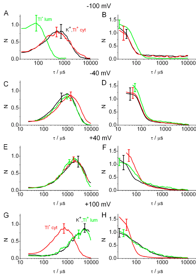
Figure 1. Dwell-time histograms of the open (A, C, E, and G) and the closed (B, D, F, and H) states obtained from MaxiK channels in the presence and absence of Tl + with the following solutions: 150 mM KNO 3 on both sides ('K + ', black), 50 mM Tl + and 100 mM K + on the luminal side (Tl + lum, green) or on the cytosolic side (Tl + cyt, red). On the opposite side there was always 150 mM KNO 3 , 2.5 mM Mg(NO 3 ) 2 and 2.5 mM Ca(NO 3 ) 2 were included in all solutions. For the sake of clarity, only representative error bars are given, which were obtained from averaging over the error bars of bins of 25% of the \tau value.
