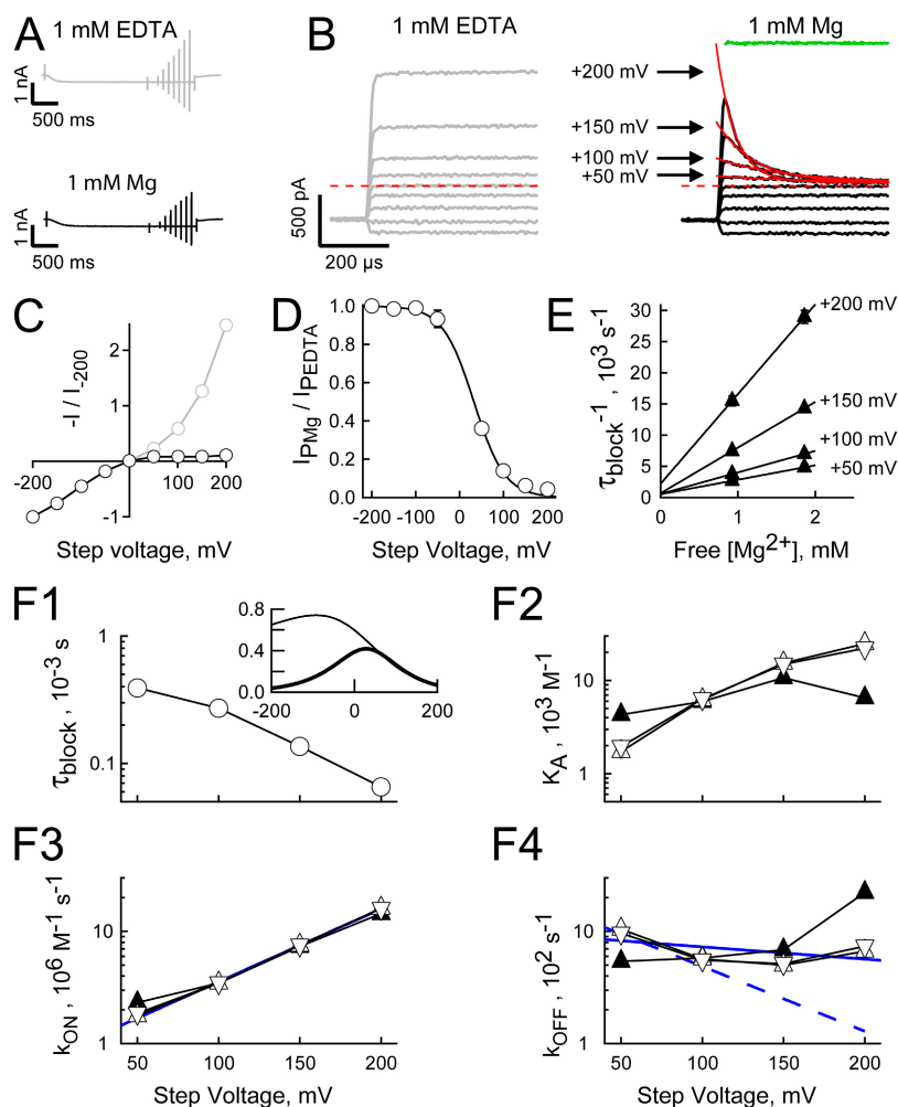
of Mg. (C) Plateau tail currents (determined at the end of test steps as shown in B) in the presence ( I_{\text{P Mg}} ) and absence ( I_{\text{P EDTA}} ) of 1 mM Mg (mean \pm SEM from nine separate recordings for each condition) plotted versus the corresponding test potential. (D) Equilibrium voltage dependence of the block by 1 mM Mg was determined by fitting Eq. 6 (smooth line) to the ratio of I_{\text{P Mg}}/I_{\text{P EDTA}} (same data as shown in C). The 95% confidence interval of this quotient was smaller than the symbol size at all voltages except -50 mV. The ratio is undefined at the reversal potential of 0 mV. (E) Plot of the inverse time constant of block at the indicated potentials as a function of the free Mg concentration. Data for low and high concentrations of Mg are mean \pm SEM of eight and four recordings acquired and analyzed as described in A–D. (F) Kinetic parameters of Mg block plotted as a function of the test potential. Parameters were determined from \tau_{\text{BLOCK}} (such as shown for 1 mM Mg in B and F1) and the steady-state current inhibition (D) according to Eqs. 1–3 based on the zero time extrapolation of the block exponential (upright open triangle) or the instantaneous current predicted from scaled amplitudes determined in the absence of internal Mg (inverted open triangle) and from 1/\tau_{\text{BLOCK}} versus free Mg concentration (E) (upright filled triangles). Solid blue lines are regressions to the data represented by the inverted open triangles. The dashed blue line represents the predicted value of k_{\text{OFF}} based on \delta_{\text{OFF}} = 0.17 (from \delta - \delta_{\text{ON}} where \delta and \delta_{\text{ON}} are 0.36 and 0.19, respectively) and k_{\text{OFF}}^0 = 1848 \text{ s}^{-1} (from the 0 mV version of Eq. 3 where k_{\text{ON}}^0 = 7.97 \times 10^5 \text{ M}^{-1} \text{ s}^{-1} and K_A^0 = 431 \text{ M}^{-1} ). The inset in F1 shows relationship of \tau_{\text{BLOCK}} to membrane voltage at 0.924 mM free Mg when k_{\text{OFF}}^0 and \delta_{\text{OFF}} are 1848 \text{s}^{-1} and 0.17 (thick line) or 936 \text{s}^{-1} and 0.03 (thin line). The ordinates are logarithmic in the main panels but linear in the inset.
