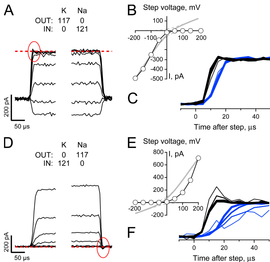
Figure 8. Na sensitivity of Mg block does not account for the collapse of conduction in a K-depleted pore. (A and D) Unblocked HCN2 currents (intracellular solution contained 1 mM EDTA and 1 mM EGTA and no added divalent cations) were collected and processed as described in Fig. 5, A and B, except the cAMP concentration was 30 \mu M and Na and K were presented biionically (with the direction of the gradients reversed in the two records as indicated). Red circles indicate a small transient present in the current collapse time course that is absent in the recovery time course. Data are representative of four and three similar recordings for A–C and D–F, respectively, with records in A–C from the same patch shown in Fig. 5, A and B. (B and E) Plateau tail current amplitudes (measured 1 ms after the beginning of each test step) plotted versus the corresponding step potential. (C and F) Expanded views of the collapse (black lines) and recovery (blue lines) of current observed when the potential was stepped between -140 mV and test potentials of +50 to +200 mV (thicker lines represent steps to more depolarized voltages). In each panel the currents have been normalized to change from 0 to 1 for both the step to, and the return from, the depolarized test potentials and each phase of the sweep shifted on the time axis so its beginning is aligned with respect to its onset.
