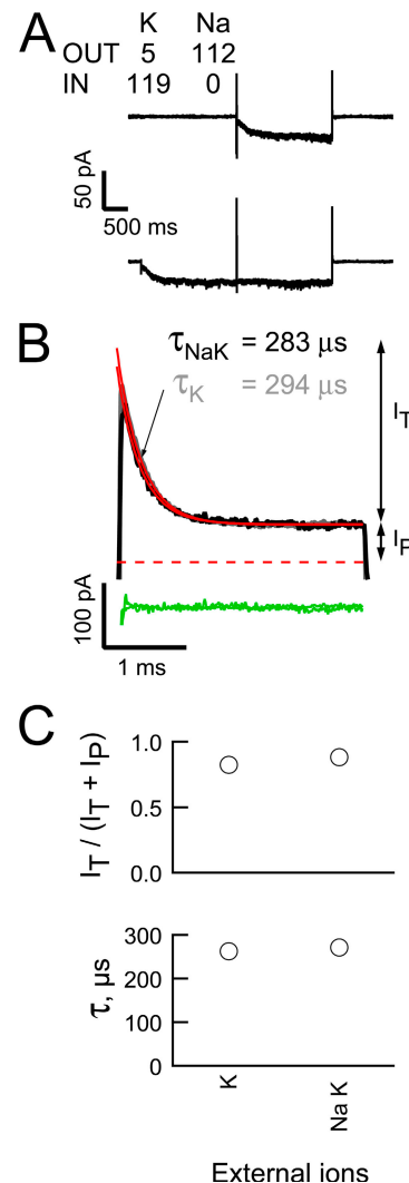
Figure 7. Mg blocks the outward HCN2 current in the presence of physiological gradients of Na and K. (A and B) Averaged sweeps (A) and subtracted predeactivation HCN2 channel +80\text{-mV} tails (B) (three and two “leak” and “active” records collected as described in Fig. 3 except for the use of quasi-physiological gradients of Na and K, black lines). In B, the gray line is the K tail shown in Fig. 4 B scaled to the amplitude of I_P of the mixed ion tail. The red and green lines represent fits of a single exponential function and the resultant residuals for the two transients. (C) Plot of the extent (top) and time constant (bottom) of block at +80\text{ mV} in the presence of elevated K or physiological levels of Na and K in the extracellular solution. Data are mean \pm SEM and range from five and two recordings, respectively.
