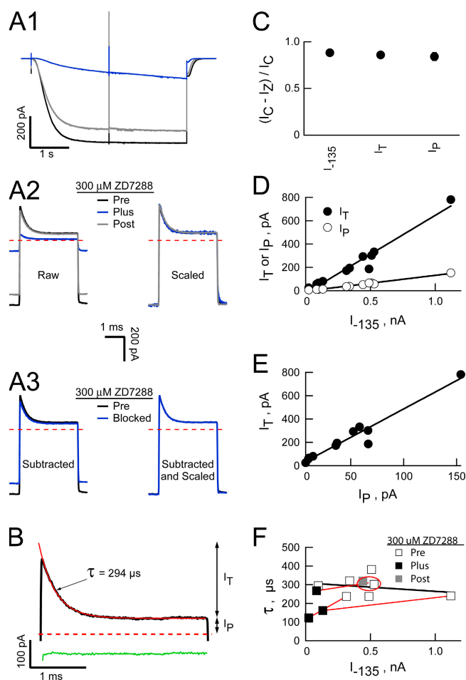
Figure 4. The transient outward current is carried by the HCN2 channels. (A1) HCN2 currents obtained before (black), during (blue), and after (gray) application of 300 \mu M ZD7288 (ionic conditions and voltage paradigms as in Fig. 3). Each trace is the average of eight sweeps evoked in response to the 3-ms “active” protocol before subtraction of the interlaced “leak” sweeps (records not shown for simplicity). Currents were filtered and sampled at 20 and 100 kHz, respectively. (A2) Expanded views of the +80 mV sojourn following subtraction of the appropriate “leak” records before (raw) and after (scaled) scaling each trace to the amplitude of the preZD7288 -135 mV current ( I_{-135} ). (A3) ZD7288-sensitive component of the current (obtained as the difference between the leak-subtracted pre and plus ZD7288 records in “A2, raw”) is shown before (subtracted) and after (subtracted and scaled) scaling the blocked component (blue traces) to the preZD7288 I_{-135} amplitude. (B) Outward transient in the absence of ZD7288 (black line) with superimposed fit of a single-exponential function (red line). Residuals from the fit (green line) are offset from zero for clarity. Arrows show the amplitudes of the plateau ( I_P ) and transient ( I_T ) components of the outward current. (C) Fractional ZD7288 inhibition of I_{-135} , I_T , and I_P , where I_C is the control amplitude and I_Z the 300 \mu M ZD7288-resistant amplitude, respectively. Data are mean \pm SEM from three recordings acquired and analyzed as described in A and B. (D and E) Linear regressions (superimposed lines) show the amplitudes of I_T ( R^2 = 0.955 ) and I_P ( R^2 = 0.986 ) are highly correlated with that of I_{-135} (D) and with each other (E; R^2 = 0.945 ). Data are from seven independent patches. (F) Time constant of current decay at +80 mV as a function of the I_{-135} amplitude. The black line is a linear regression ( R^2 = 0.070 ) across the control data from seven independent
