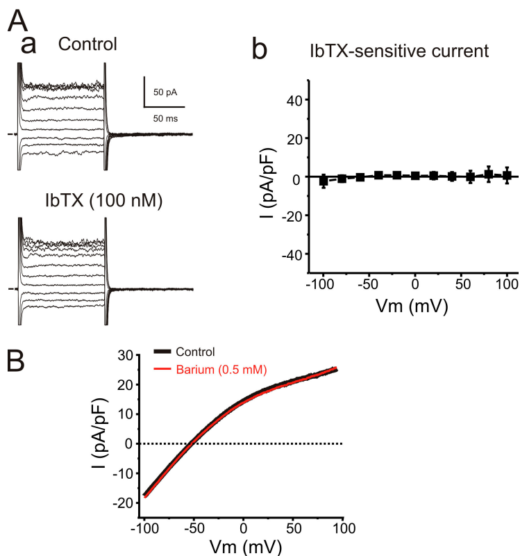
Figure 1. Functional BK_{Ca} or K_{tr} channels are not present in freshly isolated aortic endothelial cells. (Aa) Typical family of traces recorded from freshly isolated aortic endothelial cells dialyzed with a pipette solution containing 1 mM Mg^{2+} and 3 \mu M Ca^{2+} before (Control) or following application of 100 nM IbTX. From a holding potential of -50 mV, currents were evoked by 100-ms voltage steps from -100 to +100 mV in a 10-mV increment followed by a 100-ms repolarizing step to -50 mV. (Ab) Mean IbTX-sensitive current recorded from four experiments similar to the one shown in Aa. (B) Mean ramp currents in the absence (Control, black trace) and presence (Barium, red trace) of 0.5 mM barium ( n = 5 ). These currents were elicited using 45 mM extracellular K^+ to emphasize potential K_{tr} currents. Currents were induced by a 200-ms voltage ramp protocol from -100 mV to +100 mV (HP = -60 mV).
