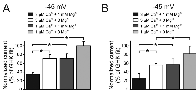
Figure 4. Comparison between native and theoretical \text{IK}_{\text{Ca}} and \text{SK}_{\text{Ca}} currents. \text{IK}_{\text{Ca}} (A) and \text{SK}_{\text{Ca}} (B) currents at -45 mV in cells dialyzed with different pipette solutions normalized to the GHK predictions depicted in Fig. 3. For 1 mM \text{Mg}^{2+} and 3 \mu\text{M Ca}^{2+} (% of GHK fit): \text{IK}_{\text{Ca}} ( 35 \pm 4 ) and \text{SK}_{\text{Ca}} ( 25 \pm 10 ); for 0 \text{Mg}^{2+} and 1 \mu\text{M Ca}^{2+} (mM): \text{IK}_{\text{Ca}} ( 71 \pm 9 ) and \text{SK}_{\text{Ca}} ( 55 \pm 5 ); for 1 mM \text{Mg}^{2+} and 3 \mu\text{M Ca}^{2+} (mM): \text{IK}_{\text{Ca}} ( 71 \pm 11 ) and \text{SK}_{\text{Ca}} ( 56 \pm 13 ); for 0 \text{Mg}^{2+} and 1 \mu\text{M Ca}^{2+} (mM): \text{IK}_{\text{Ca}} ( 99 \pm 10 ) and \text{SK}_{\text{Ca}} ( 80 \pm 17 ). *, P < 0.05 .
