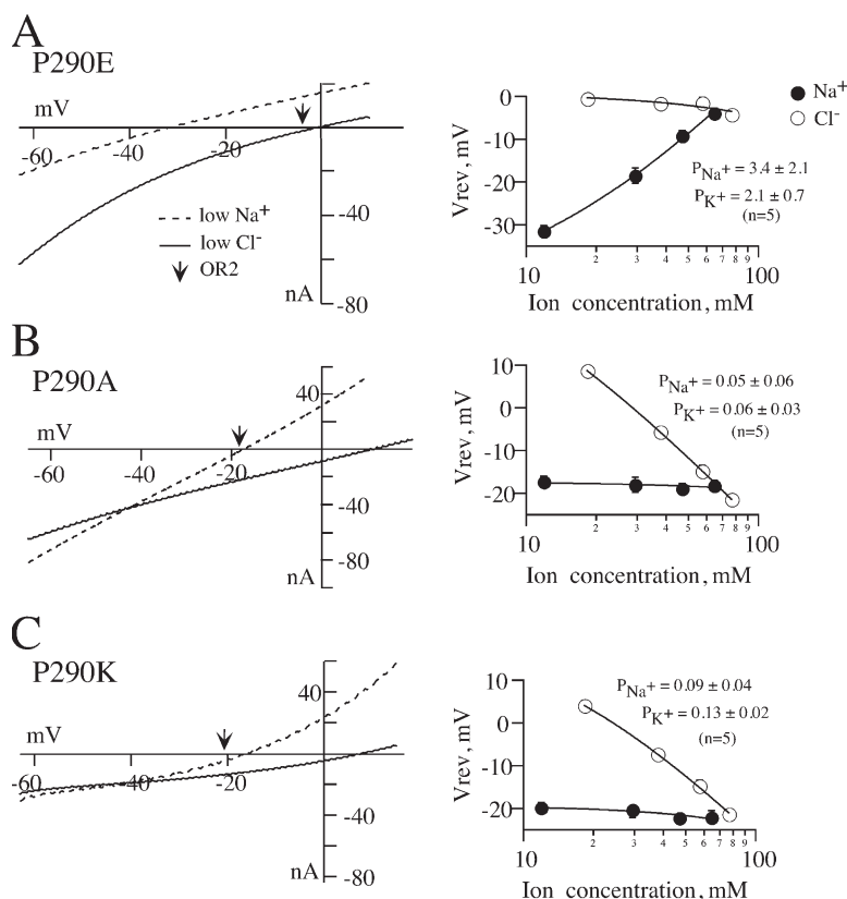
Figure 3. A negatively charged substitution at P290 ( -2' ) results in cation-preferring receptors. (A) Amplitudes of GABA-induced currents from P290E were measured at a continuously varying membrane potential using the ramp protocol described in the Materials and methods. Ramps obtained in low sodium OR2 are the dashed lines and those in low-chloride OR2 are the solid lines. The normal OR2 ramp is omitted for clarity, but the reversal potential is indicated with an arrow. For the graph on the right, reversal potentials were measured at different concentrations of sodium (solid) or chloride (open) and fit with the GHK equation (Eq. 2) to determine the relative permeability coefficients. Substitution of negatively charged glutamate for the native proline at position 290 ( -2' ) resulted in cation-preferring receptors, but receptors were chloride selective when this site was mutated to neutral alanine (B) or positively charged lysine (C).
