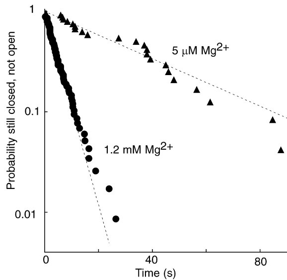
FIGURE 4. Survivor plots summarizing delays to first channel opening (i.e., closed-state dwell times following sudden introduction of 2 mM total [ATP]) from single-channel patches like those in Fig. 3. The closed times (23 delays from 9 patches at 5 \mu\text{M} \text{Mg}^{2+} ; 103 delays from 42 patches at 1.2 mM \text{Mg}^{2+} ) were ranked, fitted with a single exponential, and normalized to yield probability estimates (see MATERIALS AND METHODS) plotted here on semilogarithmic axes against dwell time. Dashed lines show least-squares fits, yielding channel opening rates of 0.22 \pm 0.003 \text{ s}^{-1} at 1.2 mM \text{Mg}^{2+} (●), and 0.03 \pm 0.003 \text{ s}^{-1} at 5 \mu\text{M} \text{Mg}^{2+} (▲).
