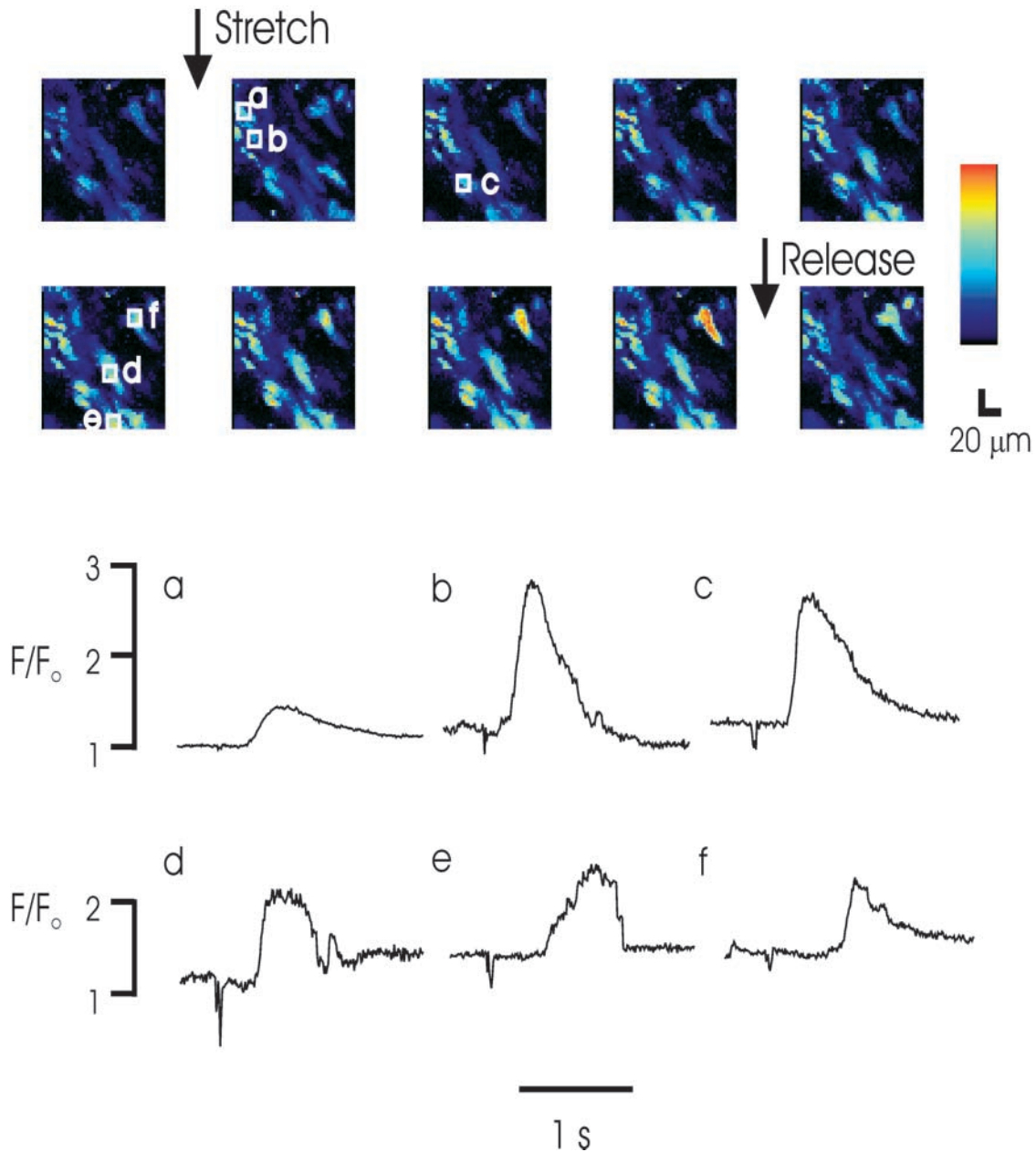
FIGURE 6. Stretch-induced Ca 2+ waves in intact mouse urinary bladder smooth muscle tissue. Above, images from a confocal time series obtained at 57.3-ms intervals. Individual boxed cell areas identify regions for which fluorescent profiles are shown below. A motion artifact identifies the point of tissue stretch on the fluorescent profiles. Note the wave of calcium evoked in single cells as the tissue is stretched. The full time series indicates evoked Ca 2+ waves within individual cells that are not transmitted to neighboring cells. Pixel size = 2.35 μM.
