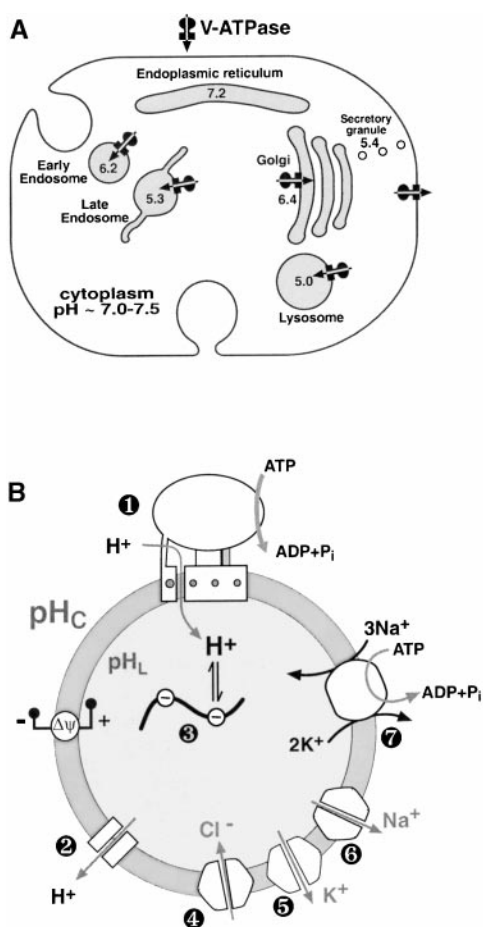
FIGURE 1. (A) A prototypical mammalian cell showing the major organelles that exhibit distinct luminal pHs along with typical pH values. These compartments tend to be in the secretory or endocytic pathways. Arrows indicate the progression along these pathways. (B) Cartoon of an organelle illustrating the principle elements influencing organelle pH regulation. (1) V-ATPase activity can be directly regulated, e.g., by dissociation of V_1 ; (2) passive proton leaks; (3) buffering by the lumenal polyelectrolyte matrix; (4) chloride channels; (5) potassium channels; (6) sodium channels; and (7) the Na,K-ATPase.
