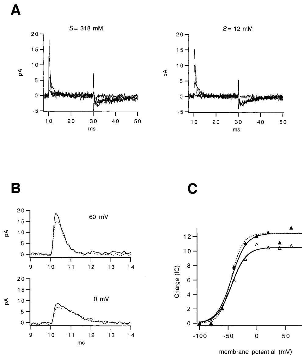
FIGURE 3. Effects of low ionic strength solutions (12 mM) on the gating currents of Shaker . (A) Gating current traces before and after perfusion of the intracellular side of a patch for depolarizations from -30 to 60 mV from a holding potential of -90 mV. (Left) Internal solution is control Cs ( S = 318 mM); (right) S = 12 mM. The spikes of the current at the beginning of the OFF gating current trace are produced by an artifact of leak subtraction. (B) Traces at the indicated potential from the same patch in A before (continuous line) and after (dotted line) perfusion with the low ionic strength solution in an expanded time scale. (C) The full Q(V) relationship. Open symbols are the charge in low ionic strength and closed symbols are the control. A reduction of \sim 16\% in the charge is apparent from this patch. The continuous curves are fits to a Boltzmann function. The dotted curve is the scaled fit to the low ionic strength data. The parameters of the fits are as follows. For S = 318 : Q_{max} = 12.4 fC, V_{0.5} = -4.4 mV, and q_g = 1.7 e_0 . For S = 12 mM: Q_{max} = 10.5 fC, V_{0.5} = -44 mV, and q_g = 1.9 e_0 .
