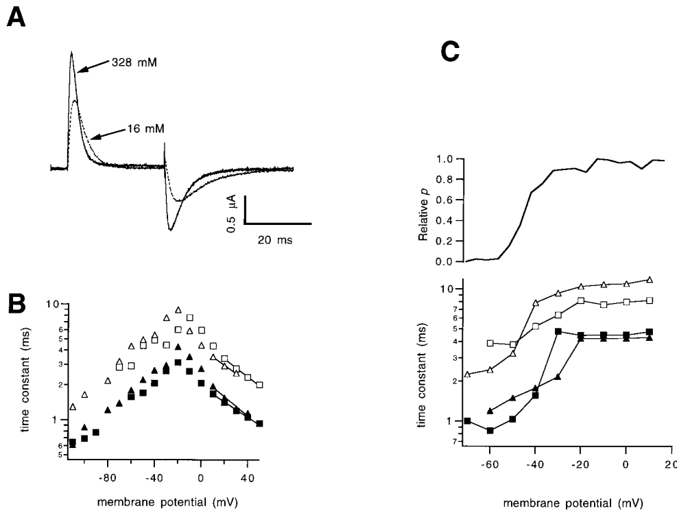
points to the function: \tau_{on}(V) = \tau_{on}(0) \cdot \exp(-q_{on}V/kT) . The values of q_{on} are as follows: (open triangles) 0.41 e_0 ; (open squares) 0.44 e_0 ; (closed triangles) 0.47 e_0 ; and (closed squares) 0.37 e_0 . (C) Time constant of decay \tau_{OFF}(V) for OFF gating currents. A single exponential was fitted to the decay phase of the current and is plotted as a function of the potential during the activation pulse. The upper panel in the figure is the relative open probability p(V) as a function of voltage, obtained from conducting channels (Sh \Delta ) recorded from a cell-attached patch in low external K^+ solution with high S (295 mM). Note that the function \tau_{OFF}(V) has a similar voltage dependence to p(V) .
