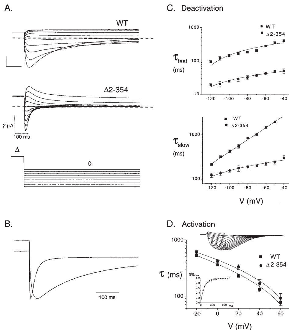
FIGURE 1. The HERG NH 2 terminus slows deactivation but does not alter activation kinetics. (A) Families of tail currents from HERG wild-type (WT) and N deletion ( \Delta 2-354 ) channels. Channels were allowed to fully activate and inactivate during a 3-s depolarizing pulse to 60 mV, only part of which is shown ( \Delta ); during a subsequent step to potentials ranging from -120 to -40 mV ( \diamond ), currents recovered from inactivation, and then deactivated. The holding potential was -80 mV. The zero current level is indicated by the dashed line. (B) Scaled tail currents evoked by a -100-mV repolarizing pulse from the experiment in A show that \Delta 2-354 channels deactivate faster than WT channels. (C) Fast (top) and slow (bottom) deactivation time constants obtained from double exponential fits to the closing phase of the tail currents plotted vs. repolarizing voltage values (see METHODS) for wild-type and \Delta 2-354 channels ( n \geq 10 ). Each point represents the mean, and the error bars are SEM for this and all subsequent figures. (D) Activation time constants for WT and \Delta 2-354 channels are plotted for different voltages. There is no significant difference between these values for WT and \Delta 2-354 channels ( P \geq 0.58 at confidence interval of 0.05 in one-way analysis of variance test). Top inset shows a series of currents evoked by the envelope of tails protocol to measure time-dependent increases in conductance, as described in METHODS, with a step to 40 mV (Trudeau et al., 1995; Wang et al., 1997); bottom inset shows exponential fit to resulting conductance vs. time plot ( n = 6 ).
