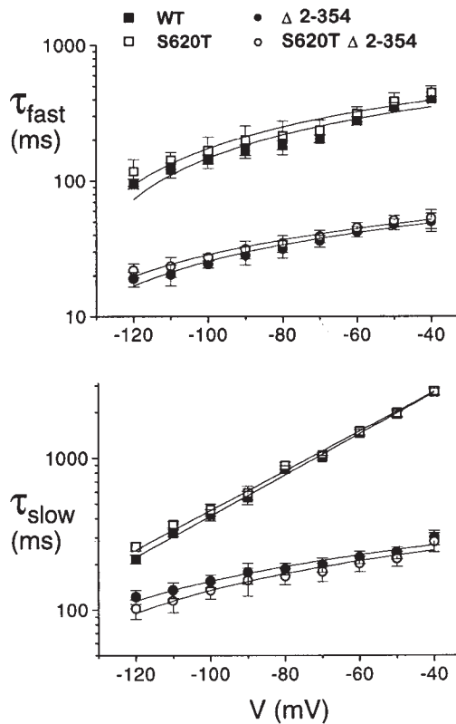
FIGURE 3. NH 2 terminus regulation of deactivation is independent of the inactivation process. (A) Scaled outward currents from S620T and S620T Δ2-354 channels show that deleting the NH 2 terminus increases deactivation rate even in the absence of C-type inactivation. (B) Fast and slow deactivation time constants for WT ( n \geq 10 ), Δ2-354 ( n \geq 10 ), S620T ( n = 6 ), and S620TΔ2-354 ( n = 6 ) channels showing that the change in deactivation rate due to deletion of the NH 2 terminus is the same in the absence of C-type inactivation as in the wild-type background.
